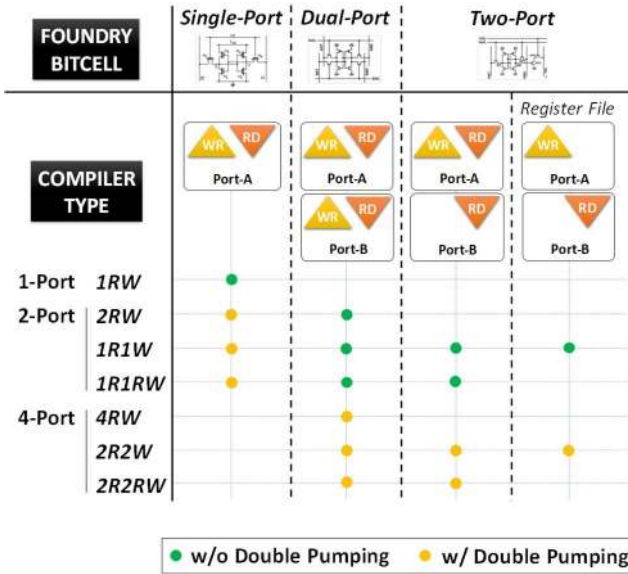
Figure 6 Possible types of SRAM compilers developed from the 3 main pushed-rule foundry bitcells ( Single-Port , Dual-Port and Two-Port ) and the use of the double pumping technique for duplicating the number of port.
