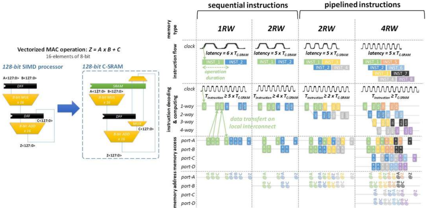
Figure 7 Chronogram of the multiply-accumulate operation ( Z = A * B + C ) performed with various C-SRAM configurations. These configurations depend on the selected SRAM type ( 1RW , 1R1W ...), the frequency ratio between C-SRAM and instruction flow and the way the instructions are performed in the digital wrapper (pipeline enabled or not).
