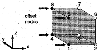
Figure 6. Definition of the four offset nodes at the x = x_{min} element face, used to define the element connectivity for the EBE method
