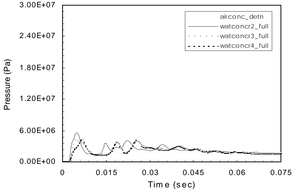
Figure 8. Pressure signatures at A1 of an explosion in a tunnel.
