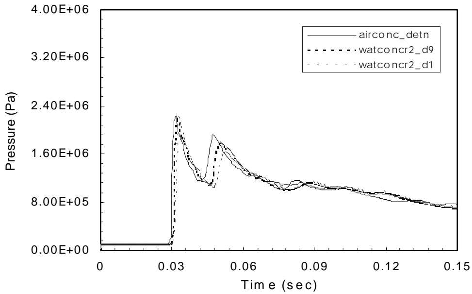
Figure 13. Pressure signatures at A3 of an explosion in a tunnel.
