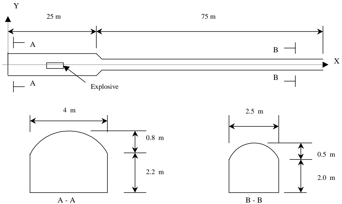
Figure 1. Layout of the tunnel.
