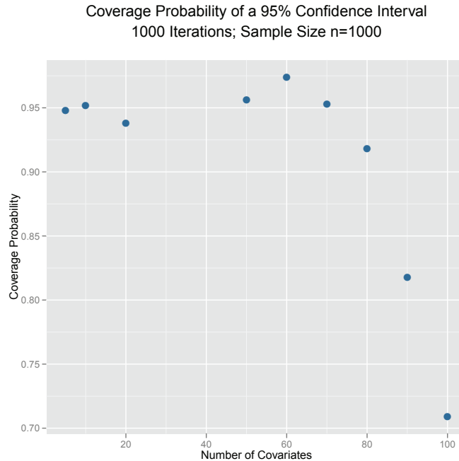
Figure 1: Coverage Probabilities, indexed by k , the number of covariates.
