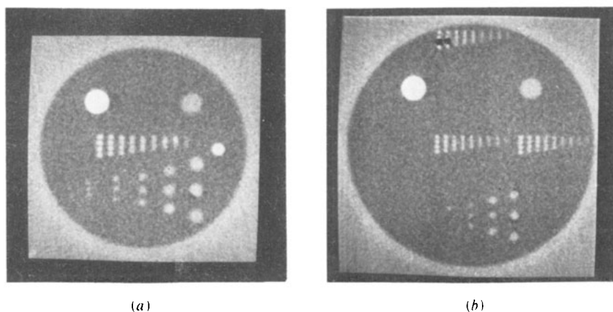
Figure 5. Proton CT reconstructions for (a) 19.3 cm and (b) 29.5 cm diameter phantoms obtained at an average dose of 0.6 cGy. The contrast of the density resolution pattern (bottom) is 1.8% with hole diameters of 12.7 mm, 9.5 mm, 6.4 mm, 4.8 mm, and 3.2 mm.
