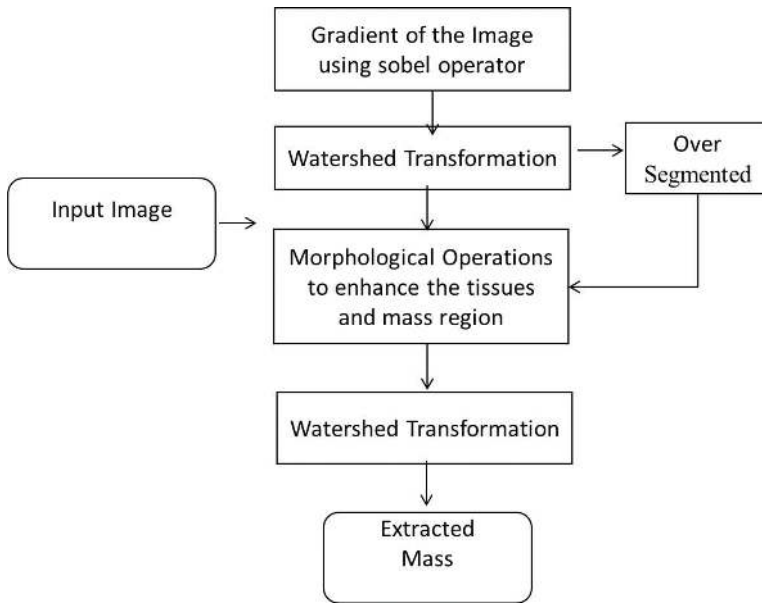
Figure 12. Steps of modified watershed segmentation technique.
