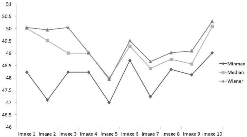
Figure 5. Comparison of different filters.
