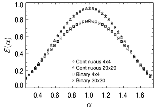
FIG. 8. Influence of phase errors on projection efficiency. Symbols indicate numerically calculated efficiencies for continuous and binary holograms encoding 4\times 4 and 20\times 20 square arrays of tweezers.
