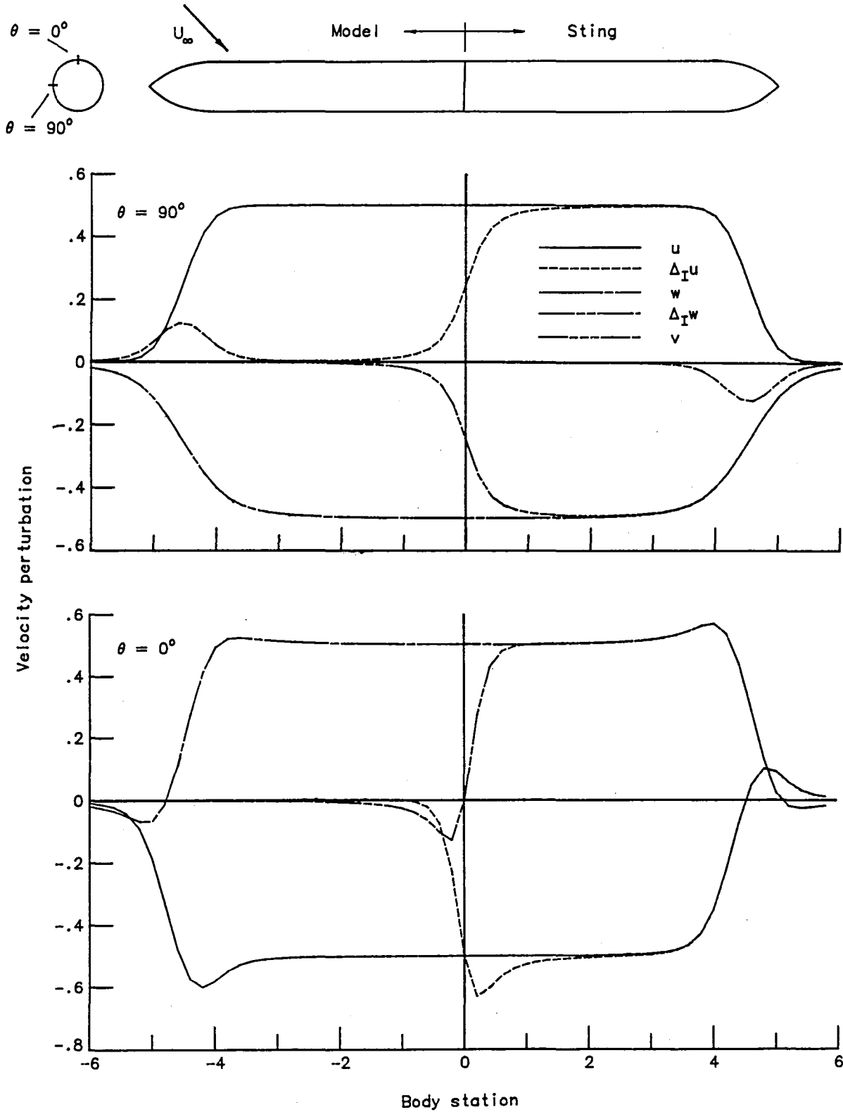
(c) Angle of attack = -45^\circ .
