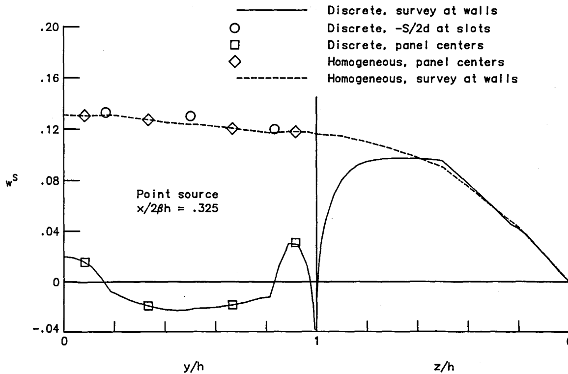
(a) Lateral and vertical distribution of vertical velocity at walls
