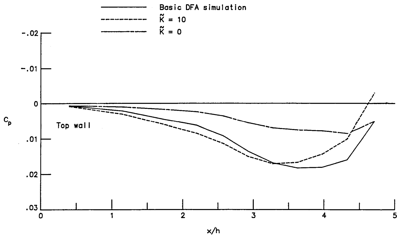
(a) Top and bottom wall pressures at y = 0.083h .
