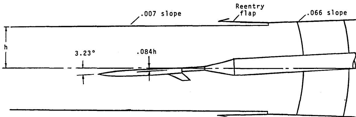
SIDE VIEW
