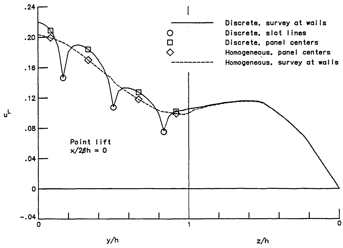
(b) Lateral and vertical distributions with point doublet and lift disturbances.
