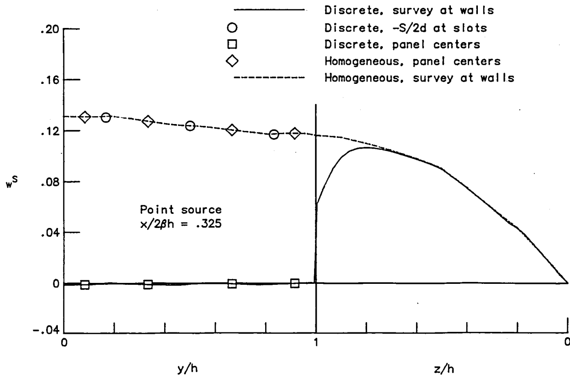
(b) Lateral and vertical distributions with point source disturbance.
