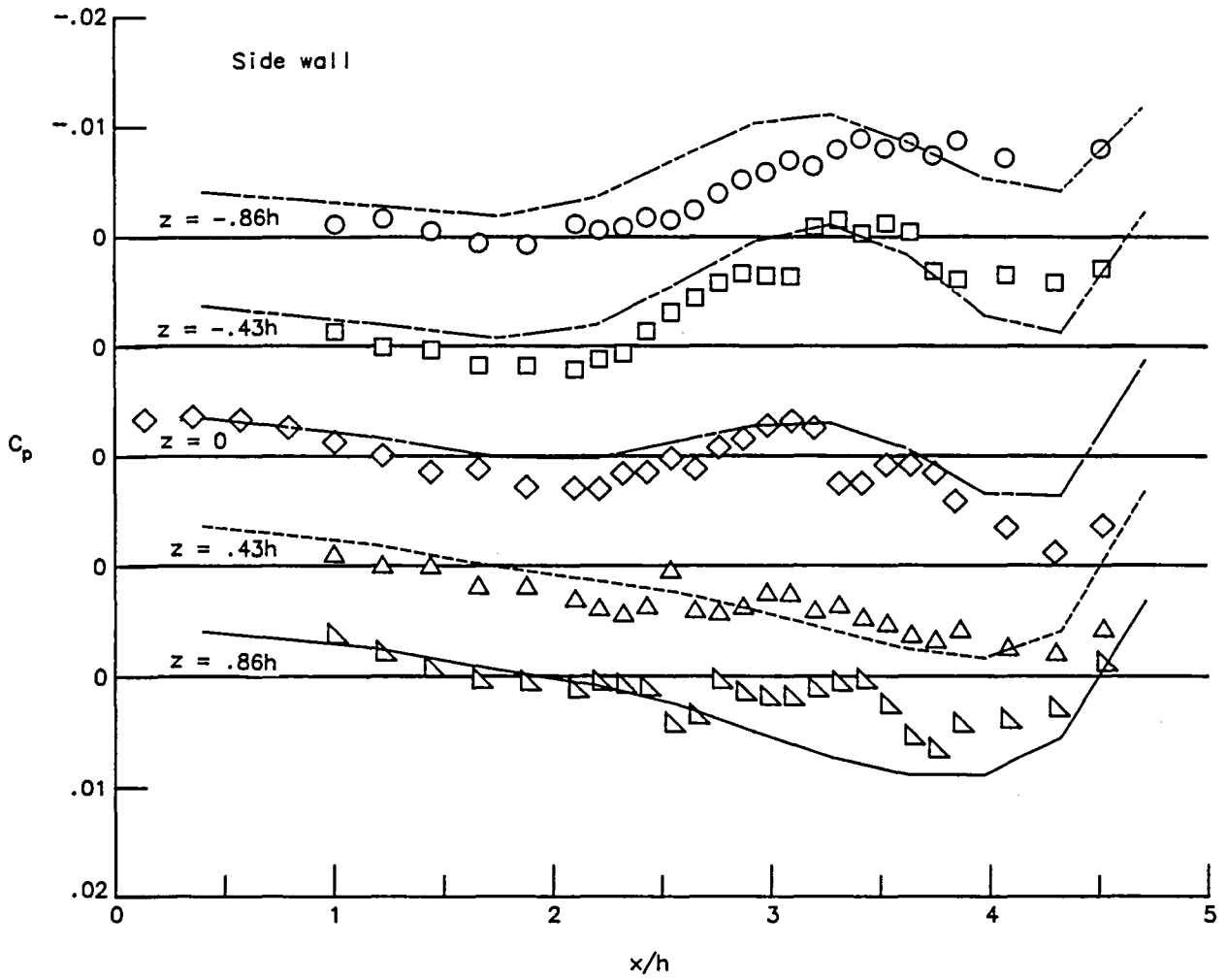
(b) Side wall pressures.
