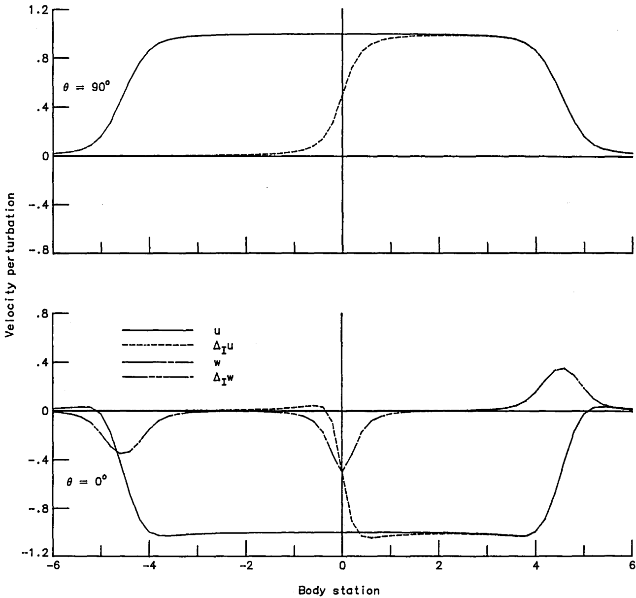
(b) Angle of attack = -90^\circ .
