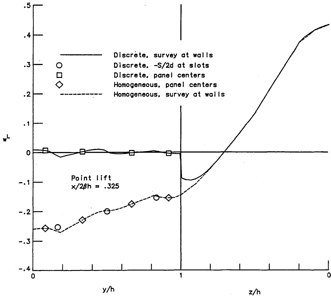
(c) Lateral and vertical distributions with point doublet and lift disturbances.
