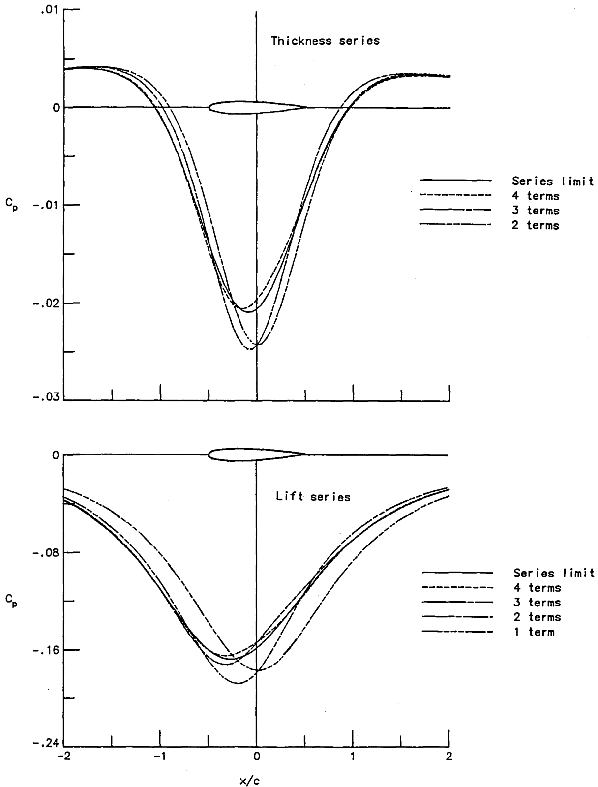
Figure 18. - Pressure coefficients induced by series representation of thickness and lift distributions of an isolated, aspect ratio 6, rectangular wing with NACA 0012 airfoil section at unit lift coefficient. Survey at y = 0, z = c .
