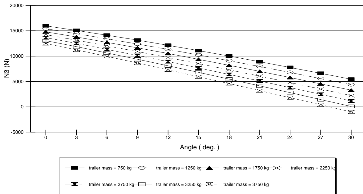
Figure 3. Soil reaction against the front wheels of tractor ( N_3 ) vs. the slope of the road (uphill) at different total mass of the trailer.
