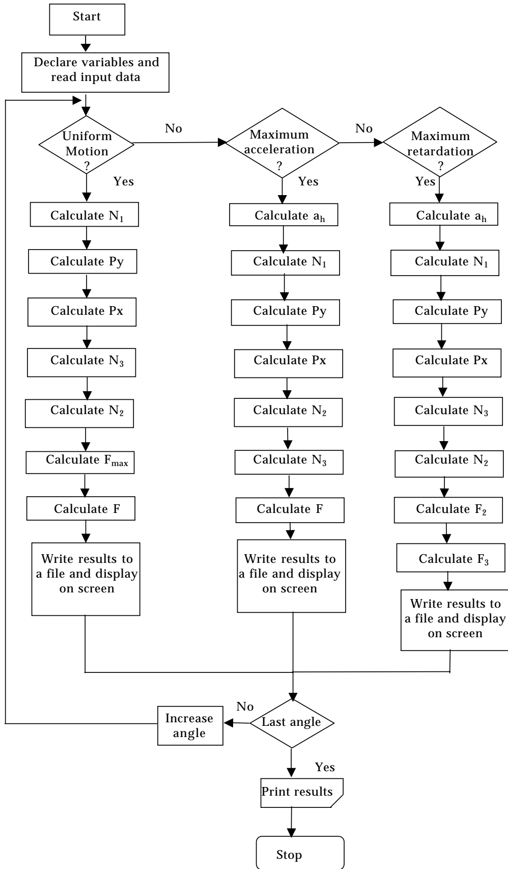
Figure 2. Flow chart of the program developed in this study.
