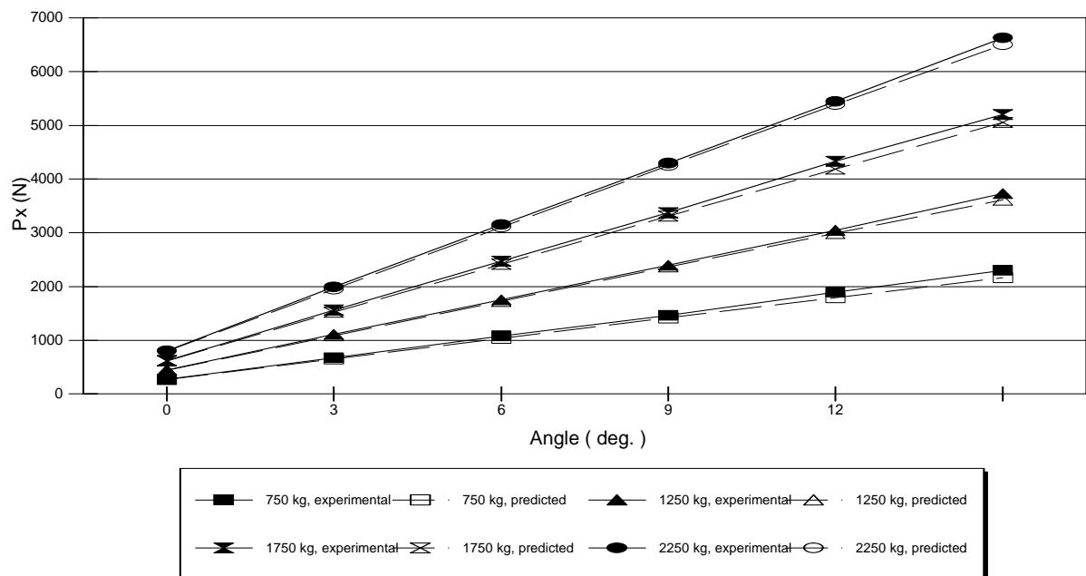
Figure 13. Measured and predicted parallel component of the drawbar pull ( P_x ) vs. the slope of the road (uphill) at different total mass of the trailer.
