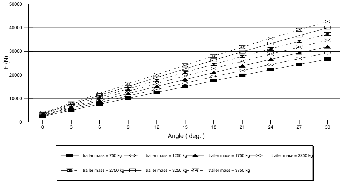
Figure 4. Traction force (F) vs. the slope of the road (uphill) at different total mass of the trailer.
