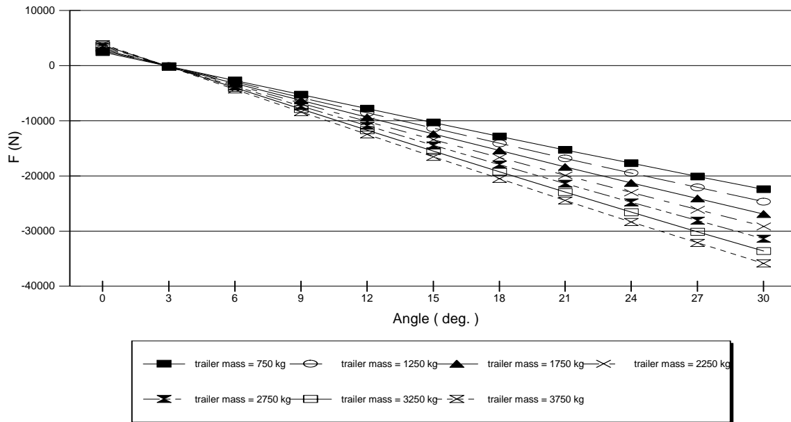
Figure 10. Traction force (F) vs. the slope of the road (downhill) at different total mass of the trailer.
