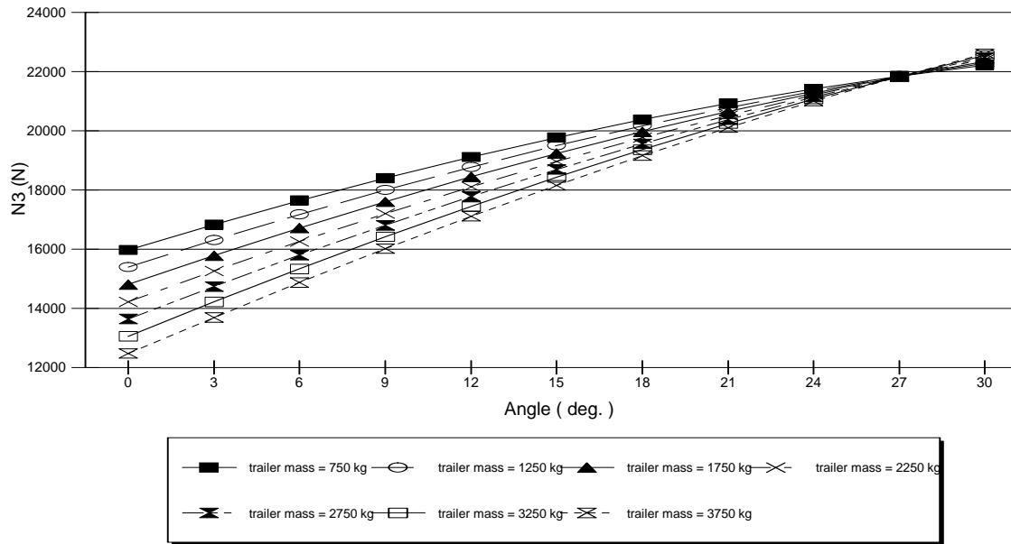
Figure 8. Soil reaction against the front wheels ( N_3 ) vs. the slope of the road (downhill) at different total mass of the trailer.
