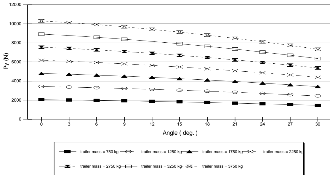
Figure 7. Normal component of the drawbar pull (Py) vs. the slope of the road (uphill) at different total mass of the trailer.
