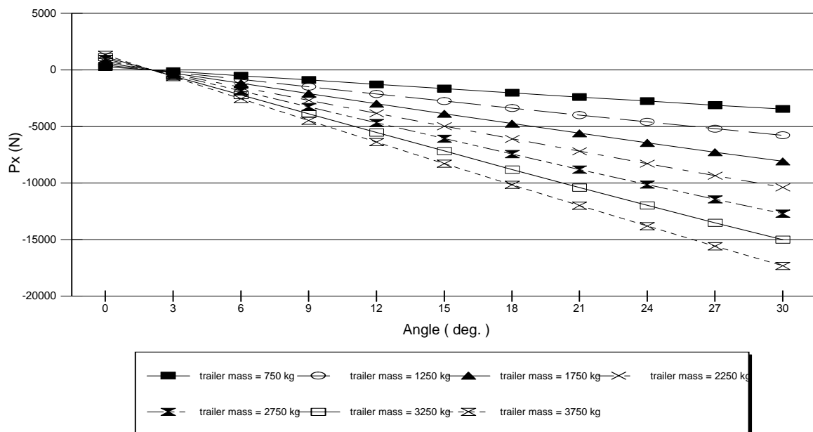
Figure 11. Parallel component of the drawbar pull (Px) vs. the slope of the road (downhill) at different total mass of the trailer.
