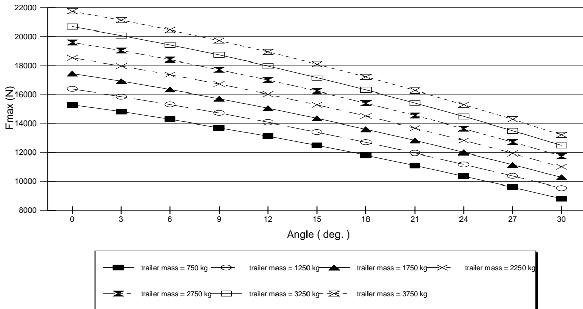
Figure 9. Maximum traction force ( F_{max} ) vs. the slope of the road (downhill) at different total mass of the trailer.
