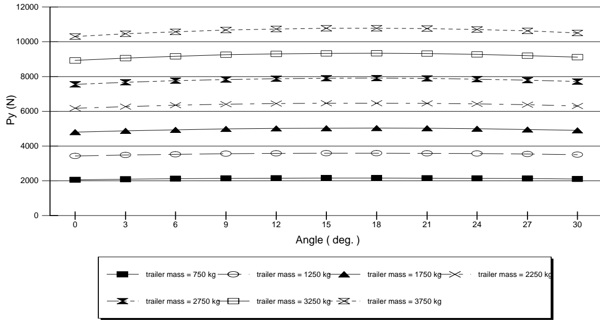
Figure 12. Normal component of the drawbar pull ( P_y ) vs. the slope of the road (downhill) at different total mass of the trailer.
