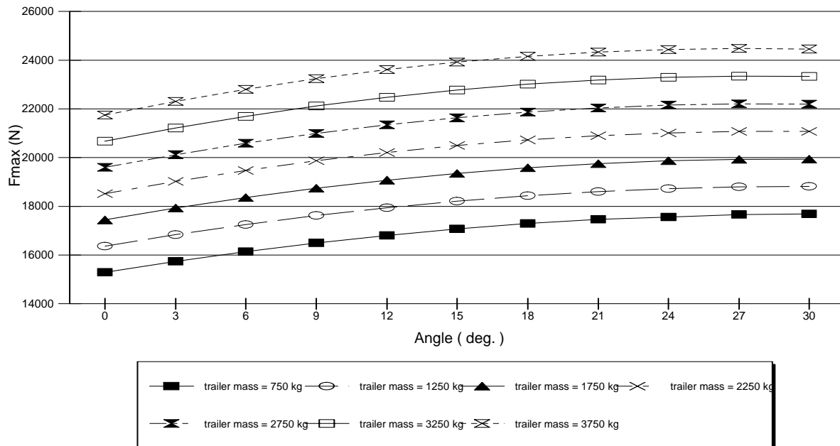
Figure 5. Maximum traction force (F max ) vs. the slope of the road (uphill) at different total mass of the trailer.
