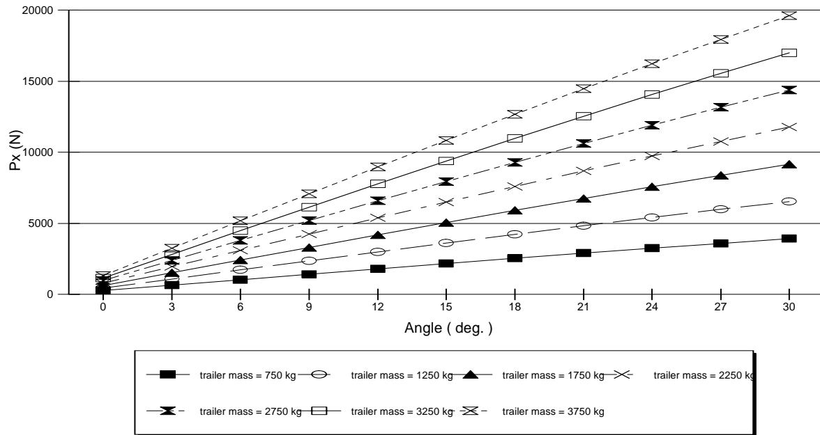
Figure 6. Parallel component of the drawbar pull (Px) vs. the slope of the road (uphill) at different total mass of the trailer.
