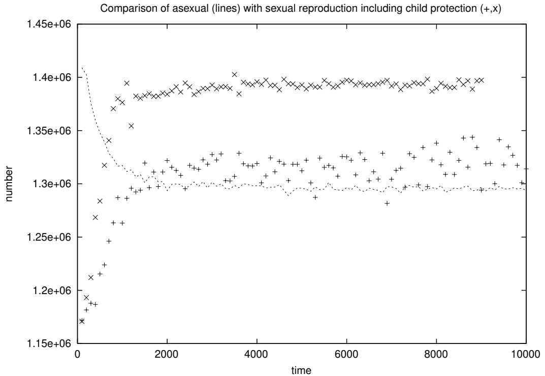
Fig. 4 – Comparison of populations, versus number of iterations, for SX with child protection (+,x), and AS (line). (For the data marked by x, females select only male partners with at most one active bad mutation.) N_{max} = 5 million; otherwise parameters as in Fig. 3.
