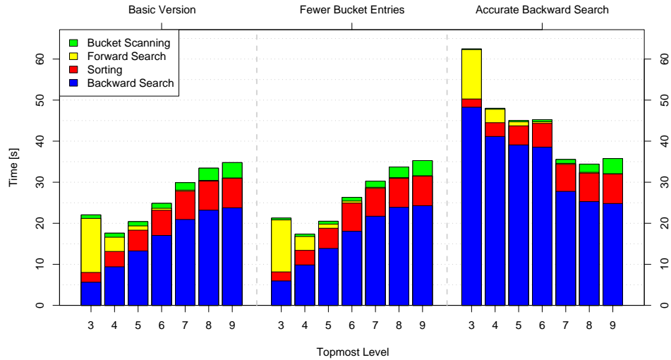
Figure 3: Performance of different algorithm variants for an asymmetric instance (100 × 32 400). The numbers on the abscissa denote the highest level K that was used in the query algorithm.
