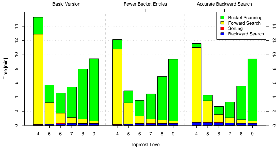
Figure 2: Performance of different algorithm variants for a large symmetric instance (20 000 × 20 000). The numbers on the abscissa denote the highest level K that was used in the query algorithm.
