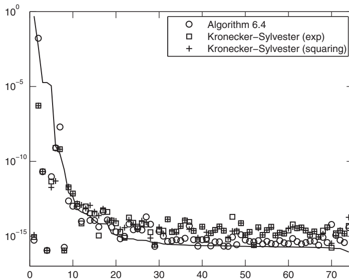
FIG. 6.1. Normwise relative errors in Fréchet derivatives L_{\text{exp}}(A, E) computed by Algorithm 6.4 and two variants of the Kronecker–Sylvester algorithm for 74 matrices A with a different random E for each A , along with estimate of \text{cond}(L_{\text{exp}}, A)u (solid line).
