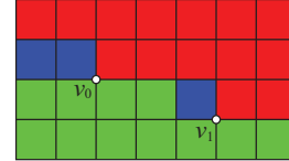
Figure 3: A small portion of the Voronoi diagram is shown. Corners v_0 and v_1 (incident by an island) both generate the same triangle with red, blue and green sites.
