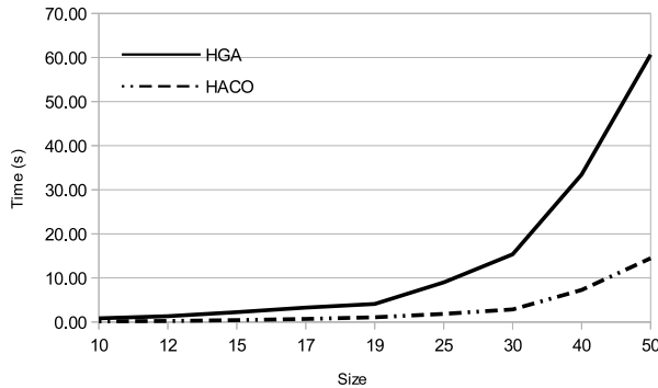
Fig. 7 Computational time results obtained for Type II cost, by problem size
