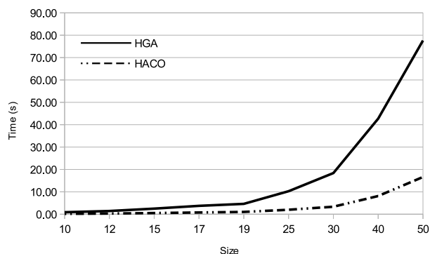
Fig. 8 Computational time results obtained for Type III cost, by problem size
