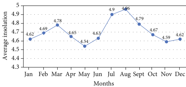
FIGURE 13: Rwanda monthly average solar insolation incident on a horizontal surface (kWh/m 2 /day). The data was collected from the National Administration of Aeronautics and Space (NASA), 2017.
