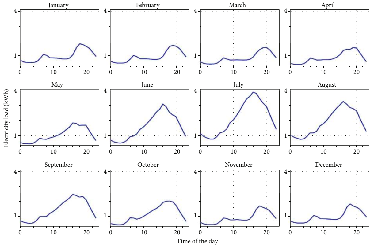
FIGURE 17: Load profile.
