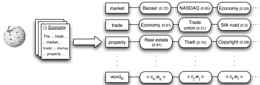
Figure 2.1: Generation of an ESA model from Wikipedia articles. The articles and words in them are processed to build a weighted inverted index, representing each word as a vector in the space of all Wikipedia concepts (articles).
