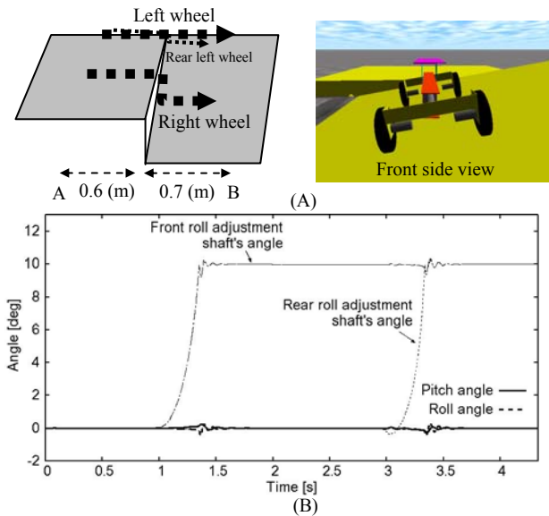
Fig.11: Simulation for the case of traversing a slope ( 10^\circ )
