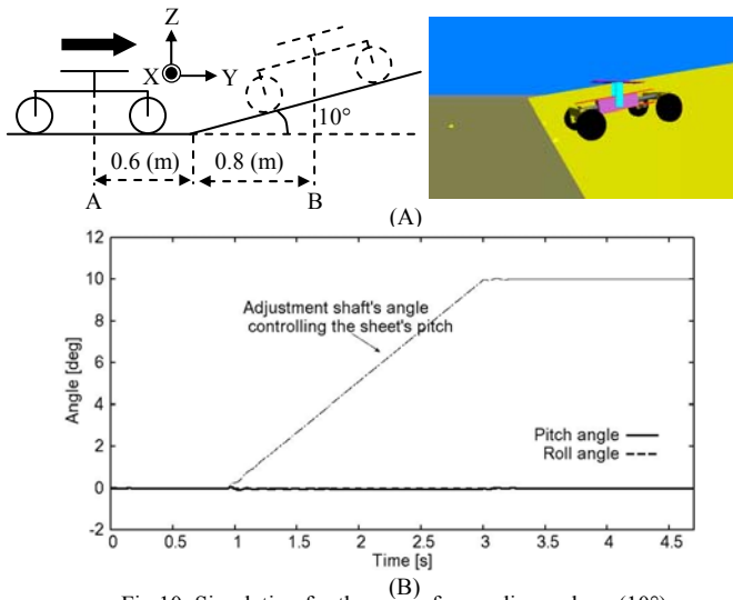
Fig.10: Simulation for the case of ascending a slope ( 10^\circ )
