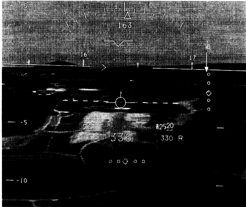
NASA Langley SVS Depiction of Approach to Asheville, NC
