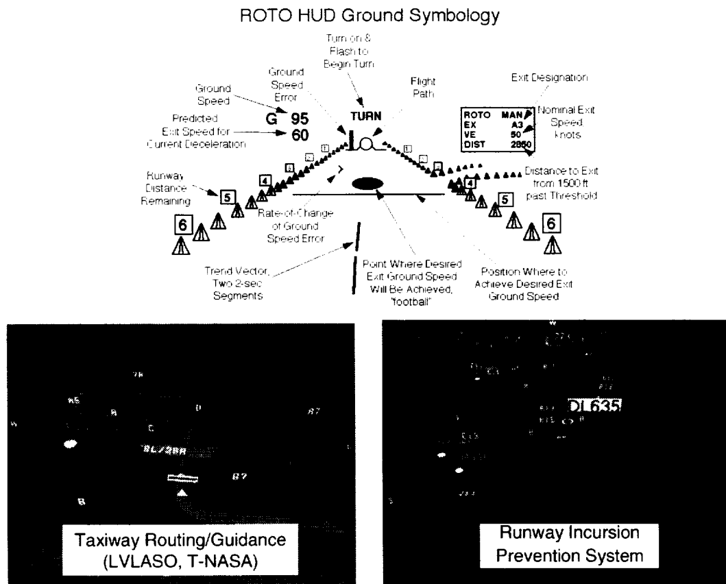
Figure 2.1 Notional Ground Operation Displays and Features
