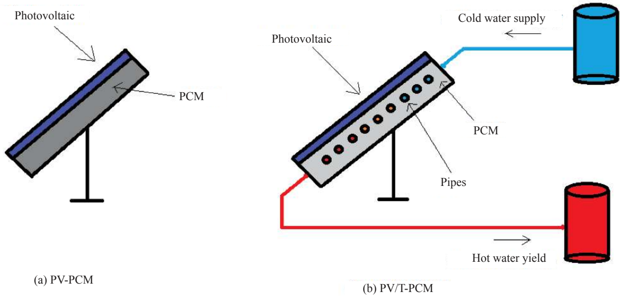
FIGURE 3. PV and PV/T-PCM cross
