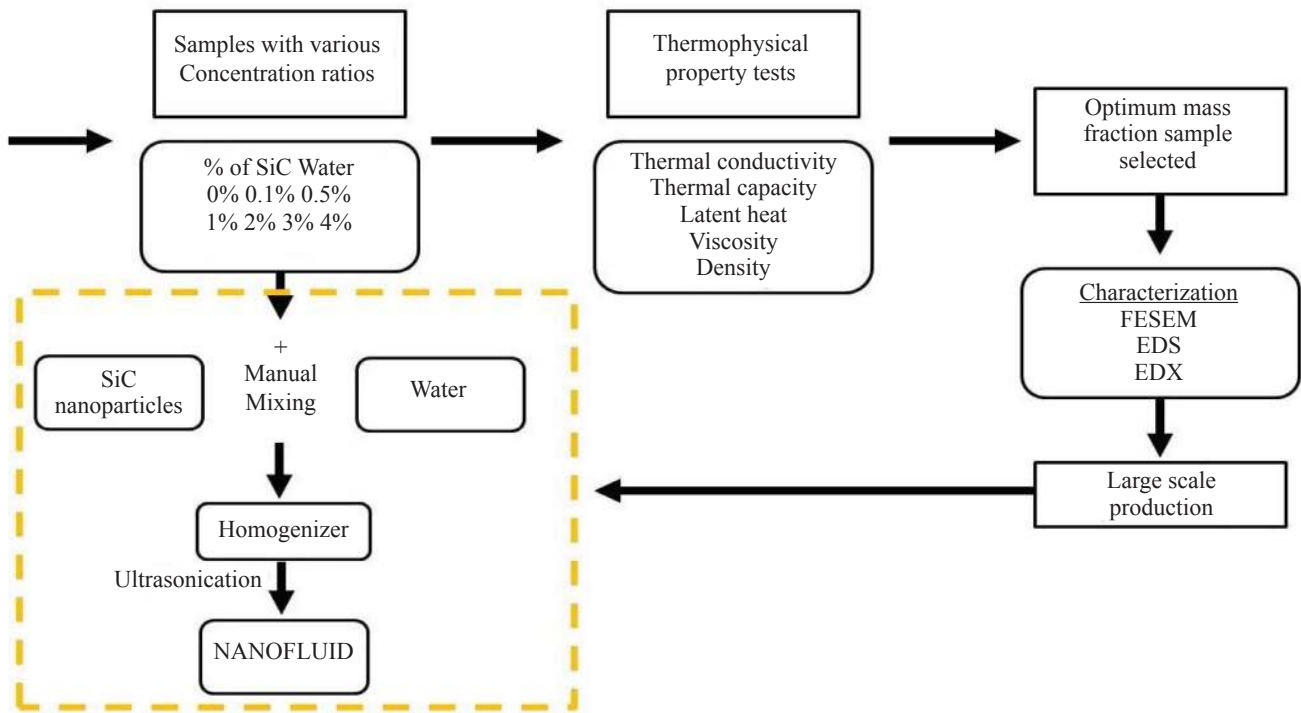
FIGURE 2. The preparation process of nanofluids (using two step method)
