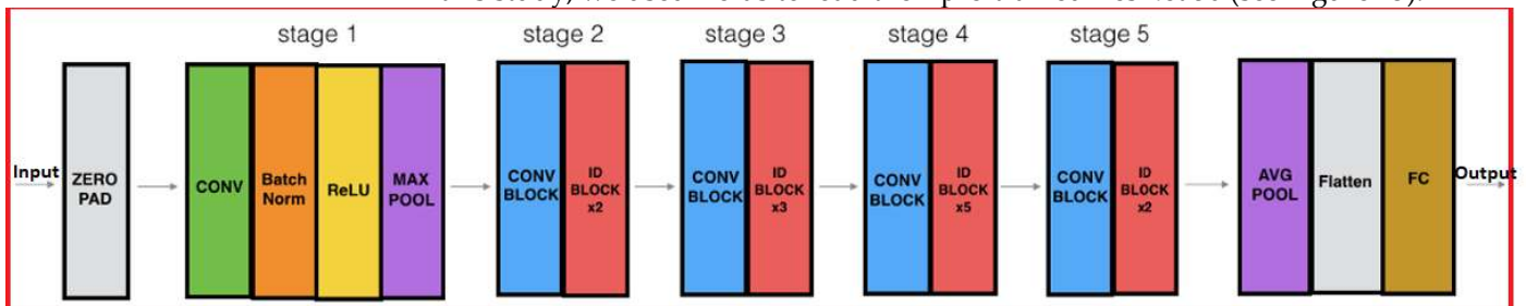
Figure 13. ResNet 50 Model
