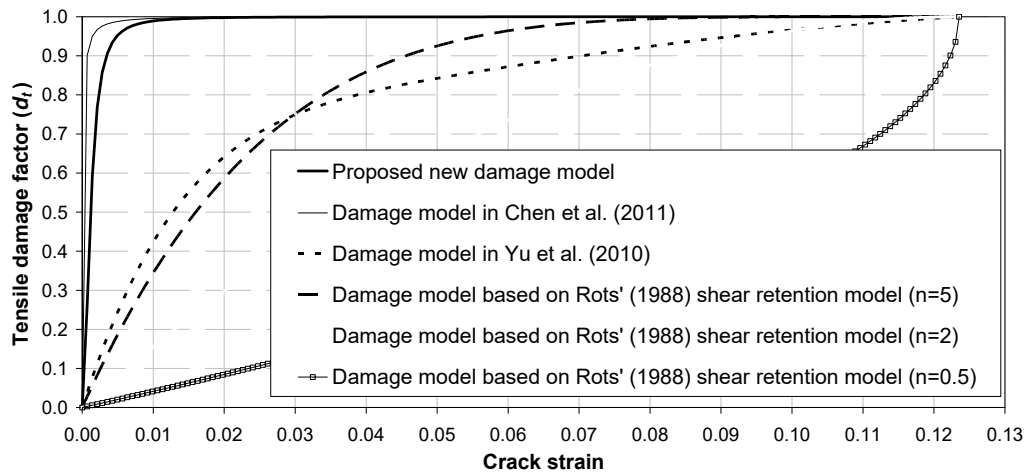
Figure 6. Tension damage models: for 1 mm element size and concrete strength as of specimen II-5 in Yao et al. (2005)
