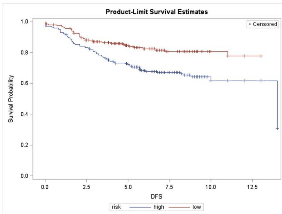
Figure 3. Disease-free survival in 408 Han Chinese breast cancer patients stratified by the 16-concurrent gene signature (Log-rank test: P < 0.001 ). X-axis: survival time in years.
