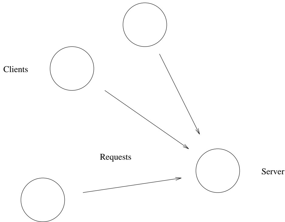
Figure 5.4 Client-server model
