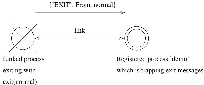
Figure 7.4 Evaluating exit(normal)
