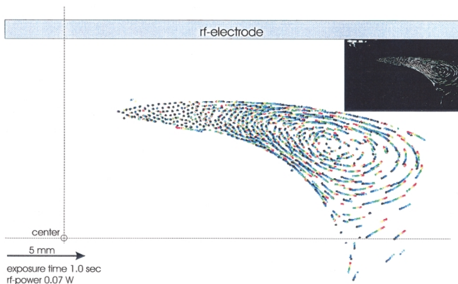
FIG. 3 (color). Cross sectional view through the colloidal plasma condensation, as in Fig. 2, but for an exposure time of 1 sec and for a rf power 0.07 W.
