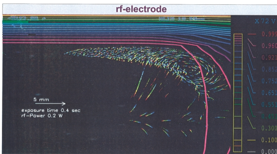
FIG. 4 (color). Cross sectional view through the colloidal plasma condensation, as in Fig. 2, but for an exposure time of 0.4 sec and for a rf power 0.20 W. Trajectories of single particles inside the void are also depicted. Note that the typical length of the “inner” trajectories (near the chamber midplane) is significantly smaller than that of the “outer” trajectories—suggesting that the force acting on the particles increases with distance from the midplane.
