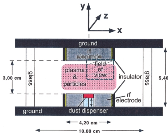
FIG. 1 (color). The space experiments were performed in a low pressure, low temperature radio-frequency (rf) discharge chamber, employing a symmetrical parallel plate reactor installed in a glass cylinder. Overall dimensions: diameter 13.6 cm, height 7 cm. The electrode dimensions are given in the figure, providing a cylindrical plasma regime of diameter \sim 5 cm and height \sim 3 cm. A piston operated dust dispenser, covered by a wire mesh of size 20 \mu m , is inserted into the center of the lower electrode. Monodisperse polymer particles of diameter 14.9 \mu m can be injected into the plasma by remote command. The gas in the plasma chamber is krypton, the operating pressure is 0.4 mbar. The rf power can be varied by telecommand to change the plasma environment. The particles are illuminated by a vertically arranged thin sheet of laser light (sheet thickness about 100 \mu m ), and visualized using a CCD video camera. Both camera and laser can be moved horizontally to obtain a 3D image of the particle cloud. The field of view is indicated—it covers roughly \frac{1}{4} of the system, which was assumed to be cylindrically symmetric.
