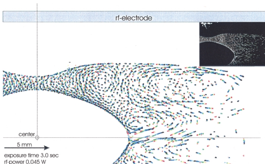
FIG. 2 (color). Cross sectional view through the colloidal plasma condensation in microgravity (TEXUS 35 rocket flight). The position of the upper rf electrode, the axis of the chamber and the midplane between the electrodes are indicated (see viewing geometry of Fig. 1). The rf power was 0.045 W and 150 video images with a total exposure of 3.0 sec are combined and color coded, thus tracing the particle trajectories (beginning with “red”). In the inset the original video image is shown. Horizontal scans verified that the particle cloud is rotationally symmetric about the chamber axis, with its outer boundary following approximately the calculated equipotential surface in the rf discharge chamber. It contains about 10^6 microspheres with a characteristic mean separation of \sim 300 \mu\text{m} . In the center there is a spheroidal “void,” where no microspheres are seen.
