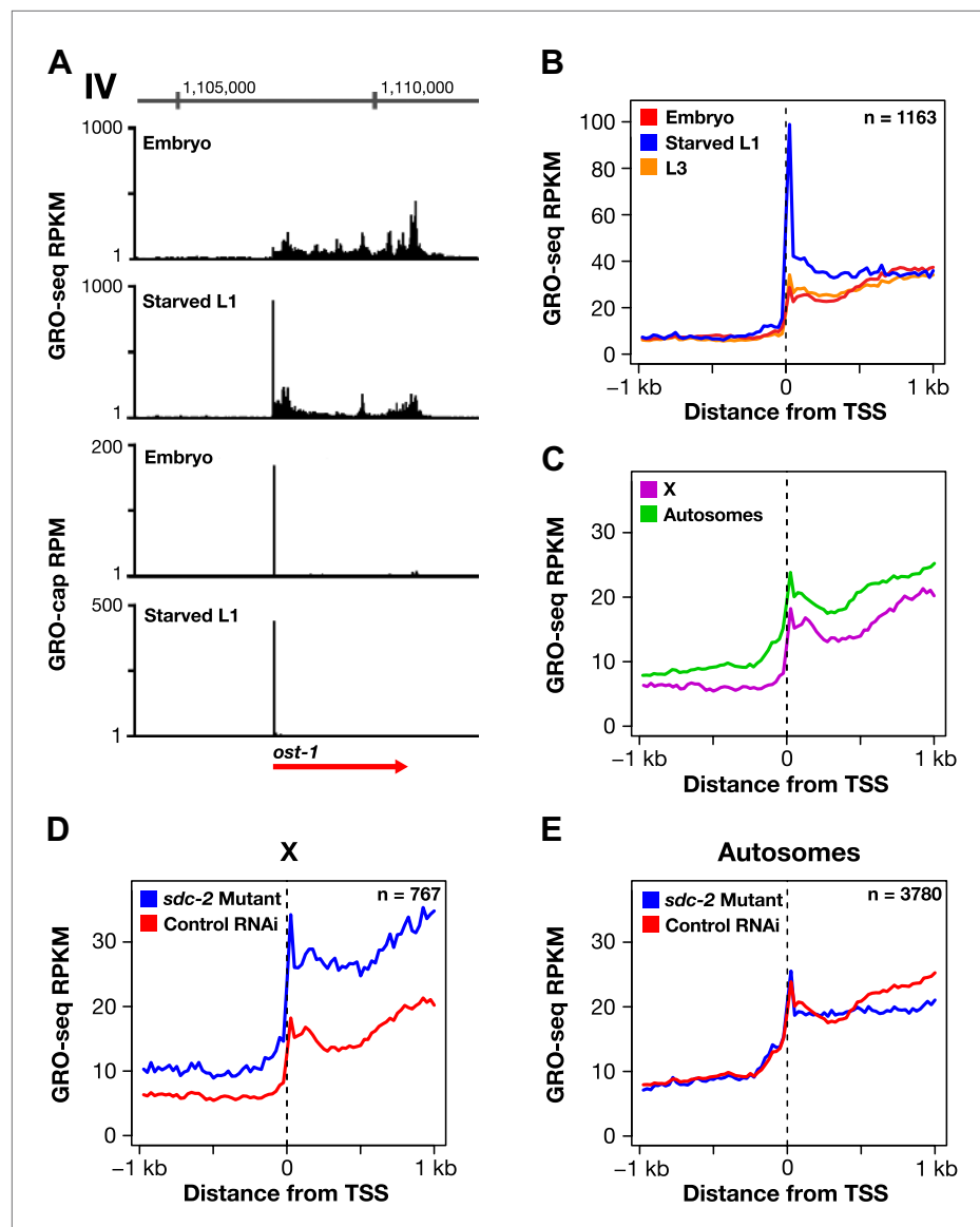
Figure 6. Promoter-proximal RNA Pol II pausing is rare in Caenorhabditis elegans and is not the target of dosage compensation. (A) GRO-seq and GRO-cap signals show that a gene not paused in embryos becomes paused in L1 larvae deprived of food. (B) Comparison of average GRO-seq signal from embryos, starved L1 larvae, and L3 larvae within 2 kb of transcription start sites (TSSs) called in all three stages shows that promoter-proximal pausing in embryos and L3s is rare compared to that in starved L1 larvae. (C) Promoter-proximal pausing is not enriched on the X chromosome relative to autosomes in embryos. If dosage compensation prevented the release of Pol II from promoter-proximal pause sites, there should be higher levels of pausing on the X chromosome. (D) and (E) The level of promoter-proximal pausing is not decreased in sdc-2 mutants compared to control embryos. If dosage compensation reduced gene expression by preventing the release of Pol II from promoter-proximal pause sites, the sdc-2 mutant should exhibit lower levels of pausing. (D) Although X-linked genes have increased expression in sdc-2 mutants, their level of pausing is not decreased. (E) The level of pausing displayed by autosomal genes is unchanged in sdc-2 mutants. RPKM: reads per kilobase per million; RPM: reads per million. DOI: 10.7554/eLife.00808.033
