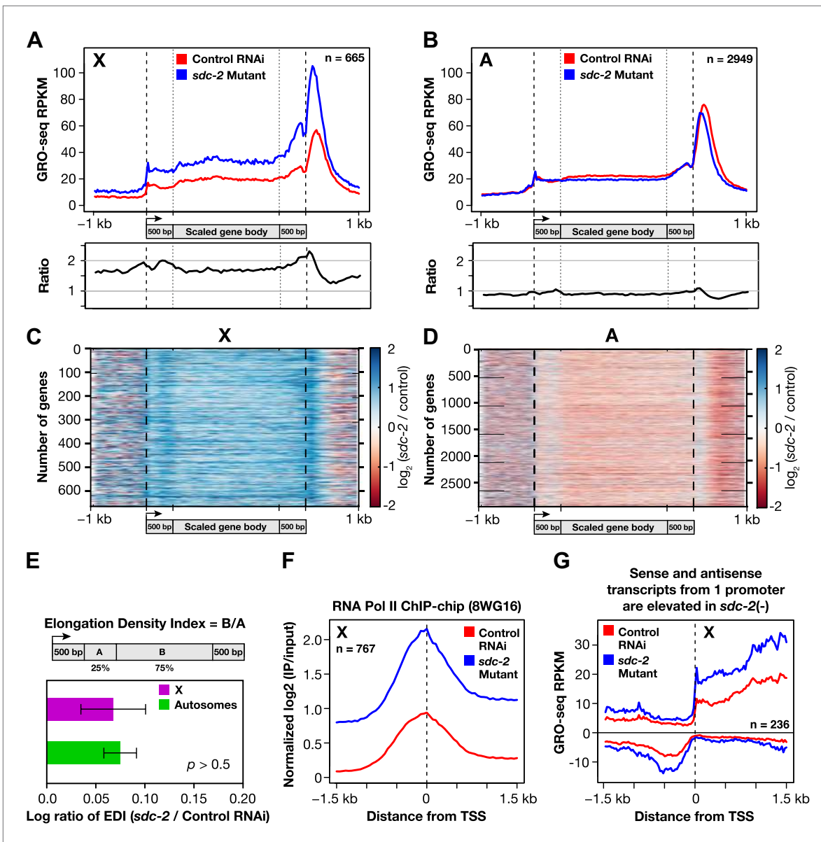
Figure 7. The DCC condensin complex reduces X-chromosome gene expression in XX embryos by restricting Pol II recruitment to promoters. (A) Uniform increase in GRO-seq signal across the length of X-linked genes results from disrupting dosage compensation. Metagenesis analysis comparing the average GRO-seq signal from 665 X-linked genes \geq 1.5 kb in control RNAi or sdc-2 mutant embryos. Genes were scaled to the same length as follows: 5' ends (-1 kb to +500 bp of the transcription start site [TSS]) and 3' ends (500 bp upstream to 1 kb downstream of 3' end) were not scaled, and the gene body was scaled to 2 kb. The signal was averaged at each base pair and then averaged across 25 bp windows. The GRO-seq signal is elevated approximately 1.6-fold across genes in sdc-2 mutant versus control RNAi embryos (below). (B) The GRO-seq signal is decreased slightly across autosomal genes in sdc-2 mutant versus RNAi control embryos. Metagenesis analysis of 2949 autosomal genes \geq 1.5 kb performed as in (D). The ratio of the GRO-seq signal in mutant versus control embryos is about 0.9. (C) Heat map shows that the GRO-seq signal is increased along the length of each X-linked gene in sdc-2 mutants. For each of 665 genes, the GRO-seq signal from mutant or control embryos was summed across 100 bp windows and the sdc-2 /control ratio was calculated for each window. The \log_2(\text{sdc-2/control}) value was plotted across the scaled gene. (D) Heat map shows that the GRO-seq signal is moderately decreased along the length of individual autosomal genes in sdc-2 mutants. For each of 2949 autosomal genes, the \log_2(\text{sdc-2/control}) value was plotted across the scaled gene as in (F). (E) Dosage compensation does not specifically affect Pol II elongation. An elongation density index was calculated for each gene greater than 2 kb in length that did not have another gene on the same strand within 1 kb of the TSS. After excluding the first and last 500 bp of the gene, the average signal across the last 75% of the remaining gene was divided by the average signal across the first 25% of the remaining gene. Ratios of the indices between the sdc-2 mutant and control RNAi embryos are not significantly different for genes on the X compared to the autosomes. Error bars represent a 95% confidence interval for the mean indices. n = 481 (X); n = 1861 (autosomes). (F) Occupancy of hypo-phosphorylated Pol II at the promoters of X-linked genes is increased in dosage compensation mutants, showing Figure 7. Continued on next page
