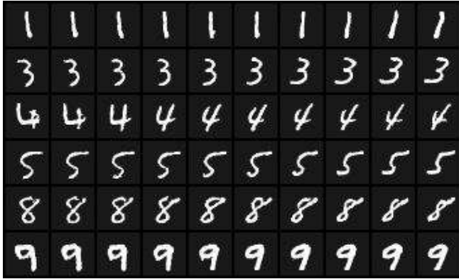
(a) Varying latent code for rotation.
