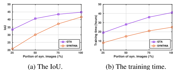
Figure 4: (a) The change of IoU w.r.t various portions of synthetic images. (b) The change of training time w.r.t various portions of synthetic images.
