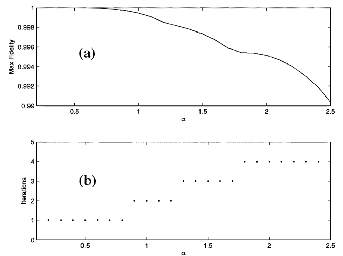
FIG. 4. (a) The maximum fidelity obtained in our scheme vs the coherent amplitude. (b) The number of iterations which gives the maximum fidelity vs the coherent amplitude.
