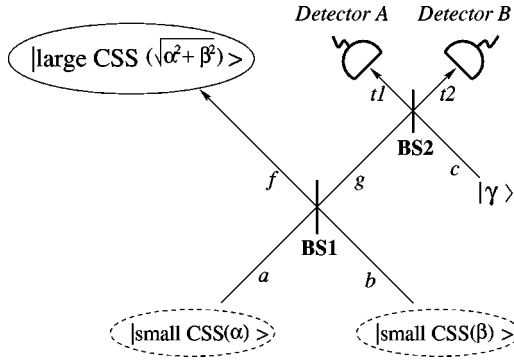
FIG. 1. A schematic of the non-deterministic CSS-amplification process. See the text for details.
