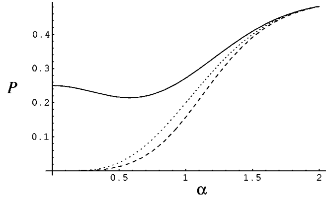
FIG. 2. The success probabilities of the CSS-amplifying process in Fig. 1 for the input fields of two identical odd CSSs (solid line), two identical even CSSs (dashed line), and even and odd CSSs (dotted line).
