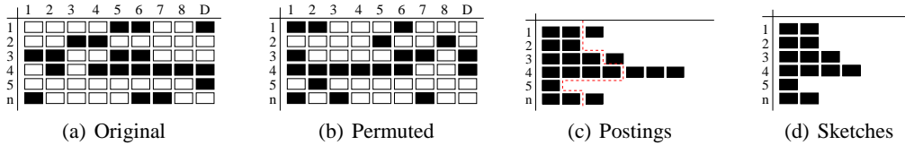
Figure 1: A global view of the sketching stage.
