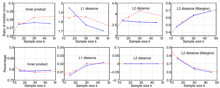
Figure 7: COREL image data.
