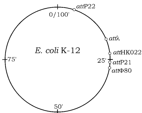
FIG. 3. Locations of chromosomal attB sites. Wild-type E. coli K-12 contains the prophage element e14 adjacent (clockwise) to attP P21 (6). Sites are based on the linkage map (3) and the positions of the appropriate attB core sequences (for attλ , gCTTtTtatActAA; for attHK022 , CTTTaggtgaa; for attP21 , tGCtGCgcCATAT; for attP22 , ATTcgtAAT-GcGAAG; for attφ80 , AACAcTTTcttAAAt; lowercase letters indicate bases that differ from the consensus [6]), in the E. coli K-12 genome sequence (4). E. coli K-12 has two attP22 sites separated by ca. 34 kb (at nucleotides 262125 and 296433 of the genome), which is consistent with their being separated by an uncharacterized phage. Furthermore, by using PCR and P22(EcoB) primers (Table 2), we have shown that the intervening sequences is absent from E. coli B, so it lacks this phage (data not shown).
