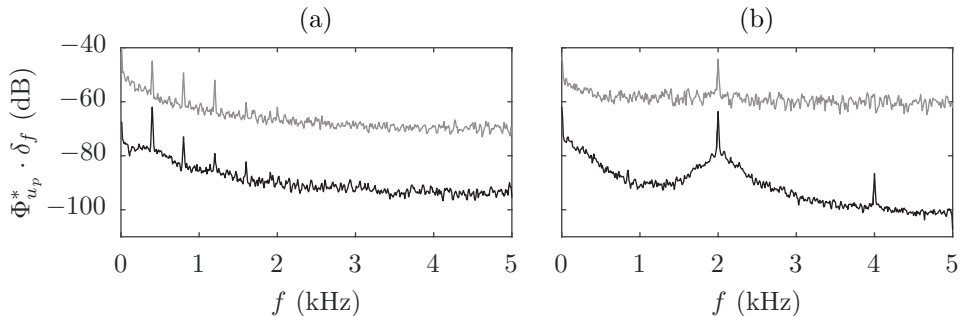
Figure 8: Non-dimensional normalised power spectra of the actuators induced velocity u_p ( \Phi_{u_p}^* \cdot \delta_f / U_\infty^2 , see equation 2.1, \delta_f=10 Hz) at the position of the markers ( x_p=1.6 mm - y_p=0.25 (grey) and 0.75 mm (black)) in figure 7 (grey curve displaced by +10dB for visualization). (a) f_f=0.4 kHz - E=3 kV, (b) f_f=2 kHz - E=3 kV.
