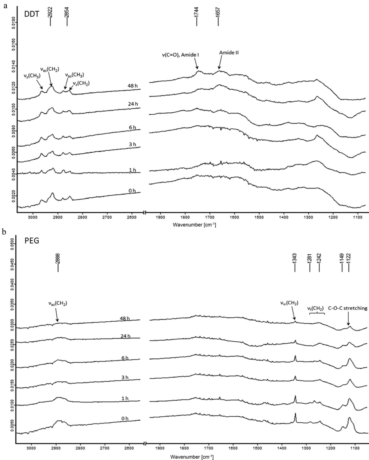
Figure S1. Infrared reflection absorption spectra (IRRAS) of the conditioning layers formed after exposure for 48 h to spore water (SP) on different self assembled monolayers.
