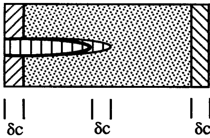
FIG. 4. Crack advance under steady state condition showing a strip of the loaded composite material far ahead of the crack front being replaced by a similar strip far behind the crack front.
