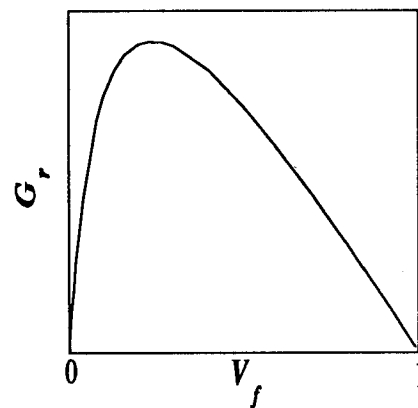
FIG. 6. Schematic representation of frictional debonding energy vs fiber volume fraction.
