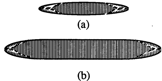
FIG. 3. (a) Short crack with bridging fibers providing closing pressure on crack flanks (b) long crack showing crack flattening under steady state condition. Elliptical crack shapes are assumed in the present analysis. The actual crack shape is probably closer to that shown schematically by the dashed lines.
