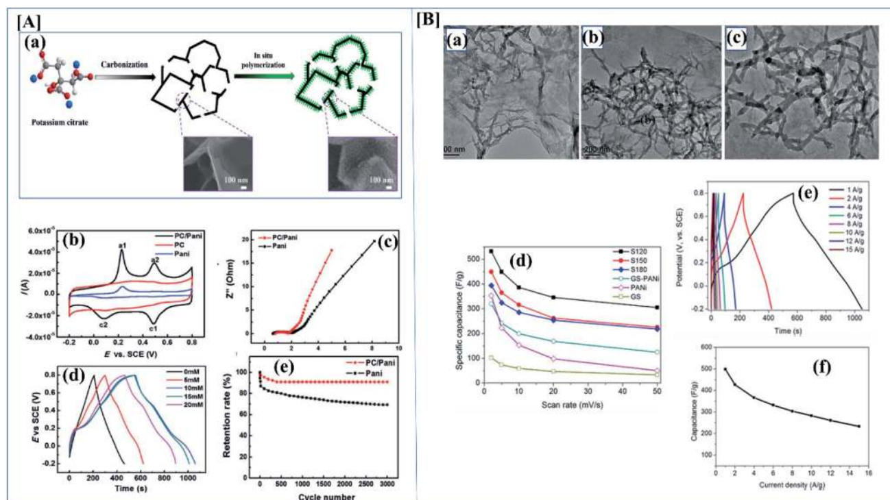
Fig. 10 [A] (a) Synthesis route for PC/PANI composite. (b) CV curves of the electrodes of PC/PANI composites, PC, and PANI at 0.05 V s -1 . (c) Nyquist plots of PC/PANI composite. (d) GCD curves of PC/PANI composites with different concentrations of aniline at 1.0 A g -1 . (e) Cycle stability of composites at a constant current density of 5.0 A g -1 (reprinted with permission, 104 copyright 2018 Wiley) [B] (a–c) TEM images of GO/PANI composites at different temperatures of 120, 150 and 180 °C. (d) Specific capacitance of GNS/PANI composites at different scan rates. (e) The GCD curves with different current densities of GO/PANI composites synthesized at 120 °C. (f) Specific capacitance of GO/PANI composites at different current densities (DOI: 10.1038/srep44562, Open source Nature).
