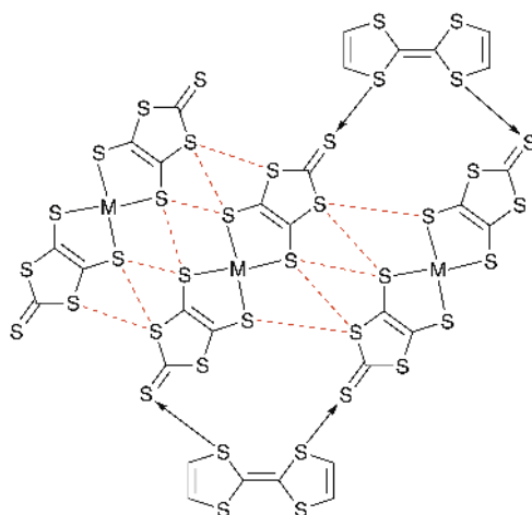
Figure 4 An illustration of the charge transfer (black arrow) between TTF and M(\text{dmit})_2 and the peripheral contacts between S atoms (red dashed line). Such van der Waals interactions yield a 2D network that avoids the instability associated with the Peierls transition. Adapted from Ref 59 .
