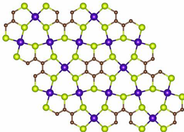
Figure 13 Predicted crystal structure of Hg(C 6 Te 6 ), following geometry relaxation at the PBEsol level of theory. The system is locally stable, adopting the same geometry as the rest of the hybrids of this class. Hg, C and Te are depicted in purple, brown and green.
