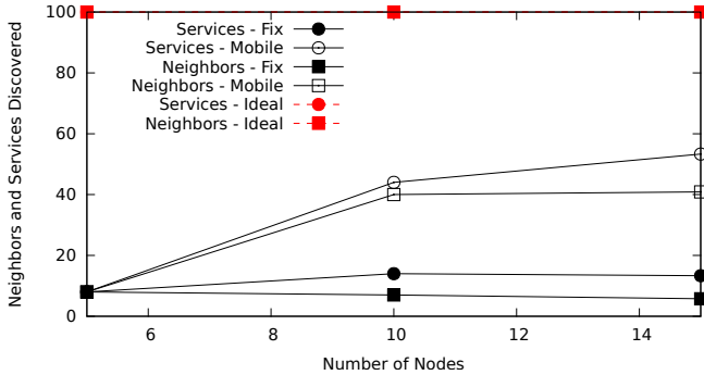
Fig. 6: Number of Nodes vs. Services and Neighbors Discovered.
