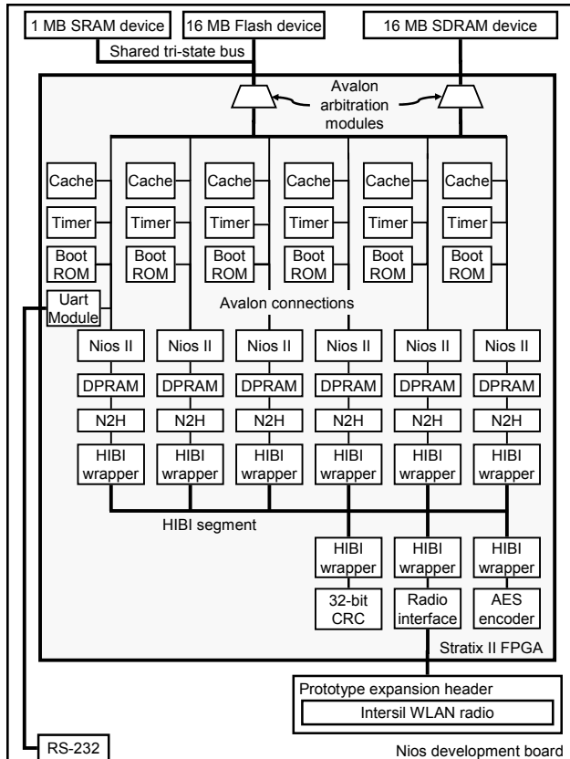
Figure 6. Platform implementation on FPGA.
