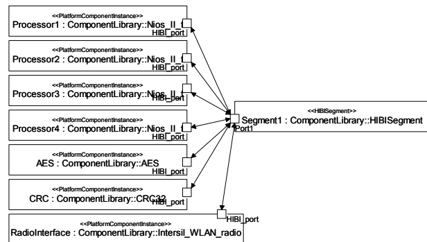
Figure 3. Architecture model of a platform instance.
