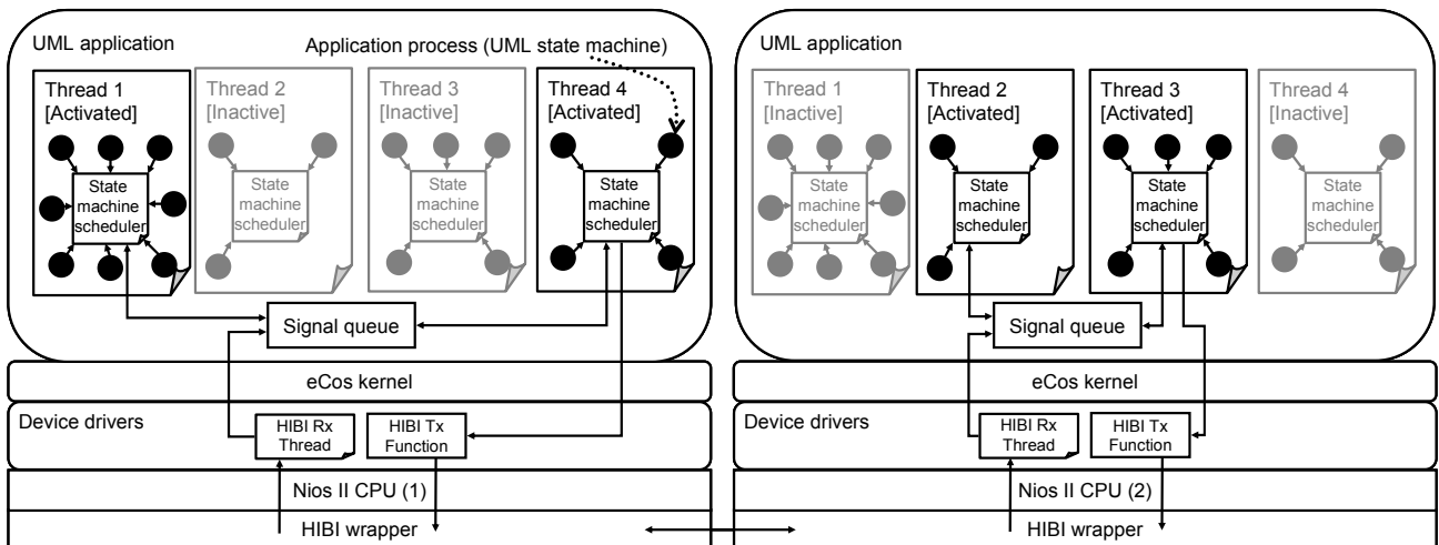
Figure 5. Application process distribution in eCos threads and signal passing arrangements.
