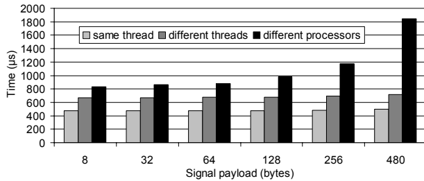
Figure 7. Delays in UML signal passing scenarios.
