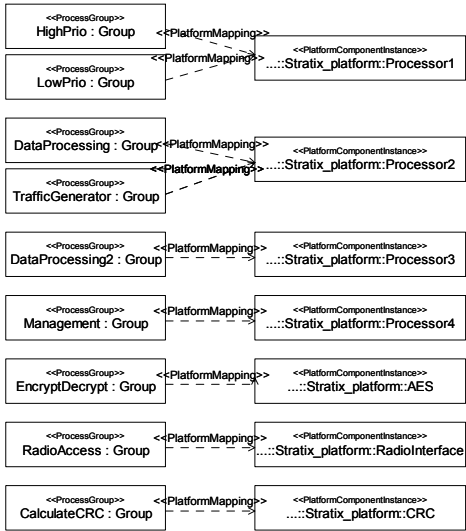
Figure 4. Mapping process groups to processing elements.
