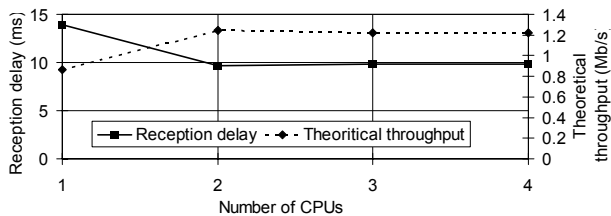
Figure 8. Reception delay and maximum throughput with different number of CPUs.
