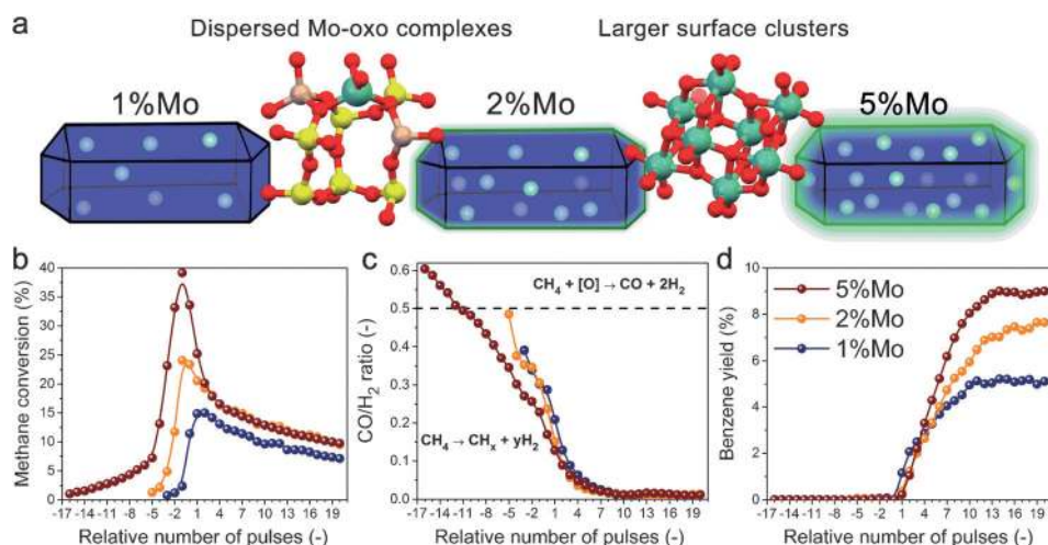
Figure 1. Representation of catalyst samples applied in this study, featuring exclusively atomically dispersed \text{Mo}^{\text{VI}} species stabilized in the zeolite pores for the 1%Mo sample and a mixture of the dispersed species and larger Mo-oxo clusters on the external surfaces of 2%Mo and 5%Mo catalysts (a). Per-pulse profiles of methane conversion (b), \text{CO}/\text{H}_2 ratio (c), and benzene yield (d), derived from MS analysis and recorded while pulsing 5 mL methane every 200 sec with 30 mL \text{min}^{-1} flow of Ar carrier.
