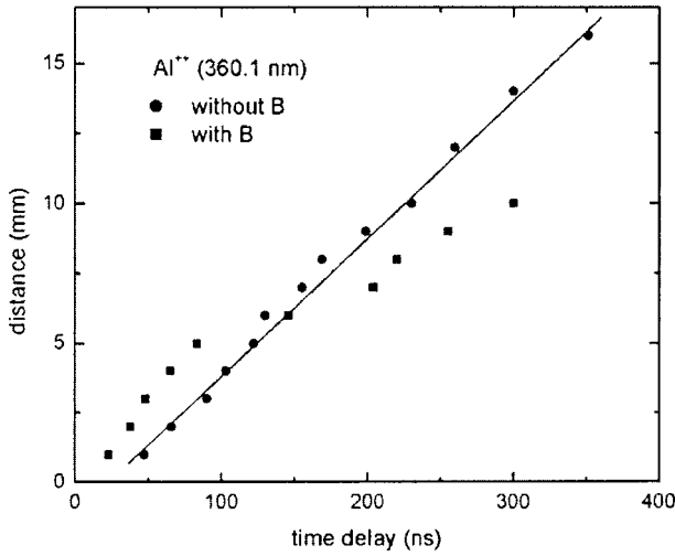
FIG. 14. R-t plot obtained from TOF profiles of Al^{2+} species with and without a magnetic field.
