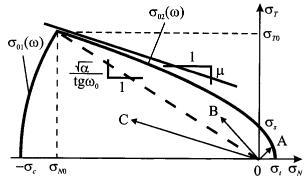
Fig. 3. Elastic domain
