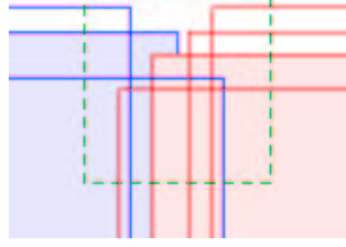
Figure 7: An illustration for Lemma 18. The tile is depicted by a green dashed square. Only the corners of squares in the corner chains are depicted. The two filled squares are the selected squares S_k and S'_\ell .
