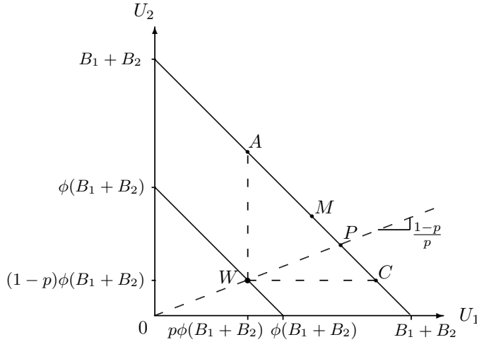
Figure 1: War and settlement outcomes
