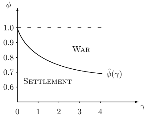
Figure 2: The critical value of \phi
