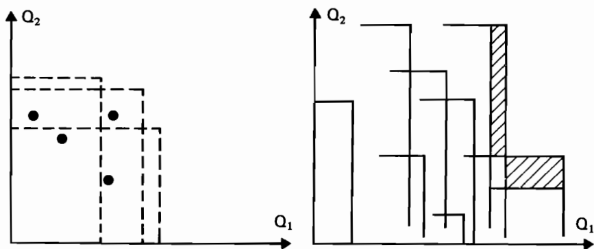
FIGURE 4.2 Example of the criterion plane and the corresponding control points for control vectors of a Pareto preference.
