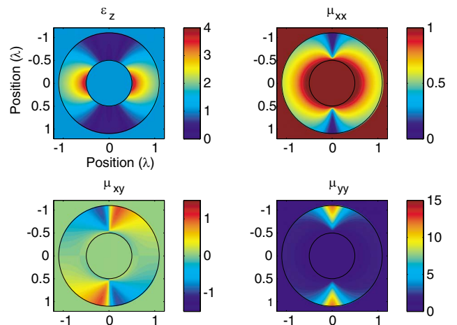
FIG. 3. (Color online) Material parameters inside the shell. For the transverse electric wave radiated by the phased array only the \epsilon_{zz} , \mu_{xx} , \mu_{xy} = \mu_{yx} , and \mu_{yy} are relevant. Very localized singularities in \mu_{xx} at r = 0.5 and x = 0 not shown on the plot.
