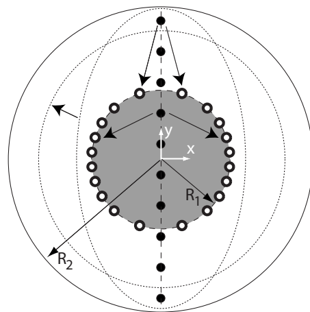
FIG. 1. The original phased array (black dots) designed to form a beam at 30^\circ in free space is modified to perform identically in the presence of the shaded cylinder. The modified design (black and white dots) is obtained using the coordinate transformation approach. Our transformation maps ellipses into circles: the dashed line maps into the dashed circle of radius R_1 , the dotted ellipse maps into the dotted circle, and the solid circle of radius R_2 maps into itself.
