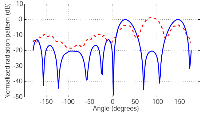
FIG. 4. (Color online) Far-field radiation patterns of the original phased array and array modified to satisfy geometrical constraints are identical (solid line). Without the anisotropic shell the radiation pattern changes significantly (dotted line). The main lobe is at 90^\circ instead of the desired 30^\circ ( 0^\circ corresponds to the direction perpendicular to the reference array).
