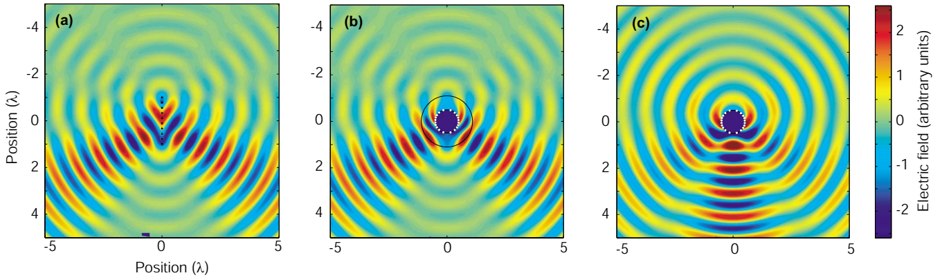
FIG. 2. (Color online) (a) Electric field produced by a phased array made of ten line sources spanning a length of 2\lambda , designed to radiate in free space at an angle of 30^\circ ; (b) Transformed phased array modified under geometrical constraints. The shell between the two cylinders is made of an inhomogeneous material designed using coordinate transformations; (c) Electric field in the absence of the shell.
