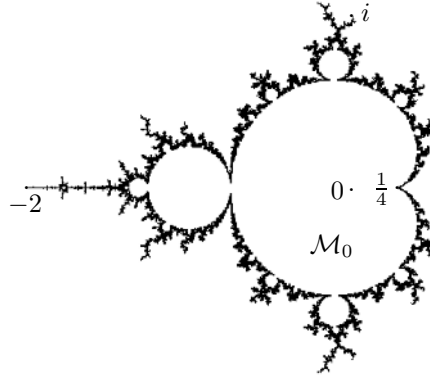
Figure 5.1: Mandelbrot set
