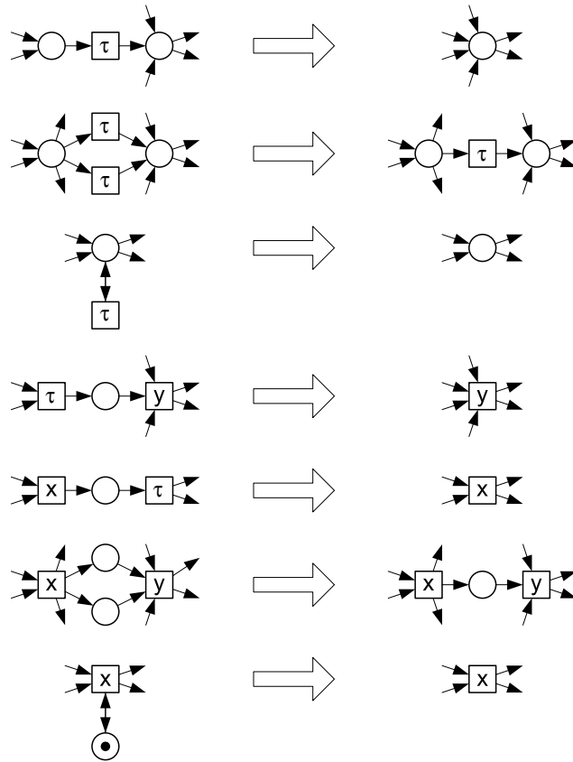
Fig. 10. Behavior preserving reduction rules used in WofBPEL.
