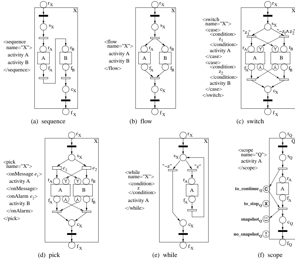
Fig. 7. Mapping structured activities.
