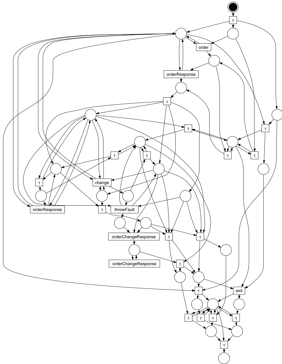
Fig. 11. The WF-net for the Supplier process.
