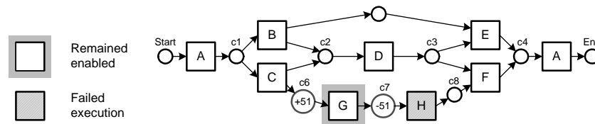
Fig. 4. Example process model after replay of event log L_2 .
