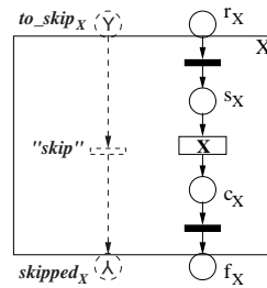
Fig. 6. A Basic activity.
