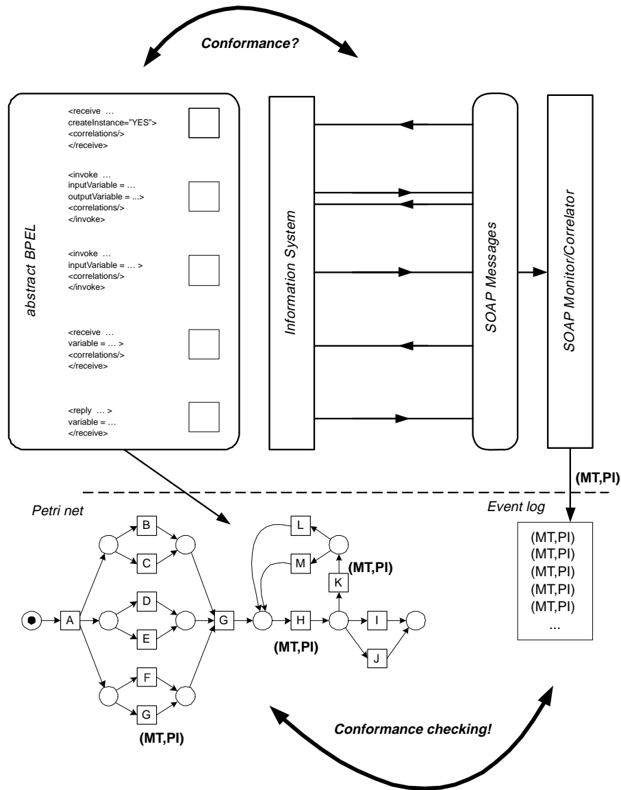
Fig. 2. Overview of the approach. The top level shows the process model in BPEL and the recorded behavior in the form of SOAP messages. The BPEL specification is mapped onto Petri nets and the SOAP messages are put in an event log. Finally, both are compared using conformance checking.
