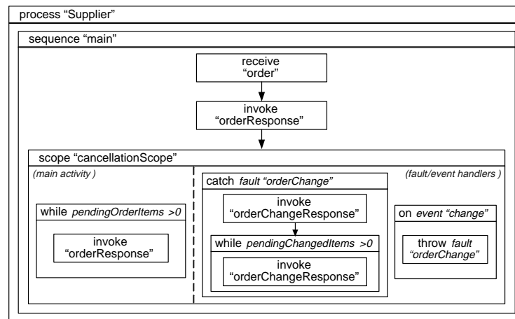
Fig. 5. An abstract view of the Supplier process.
