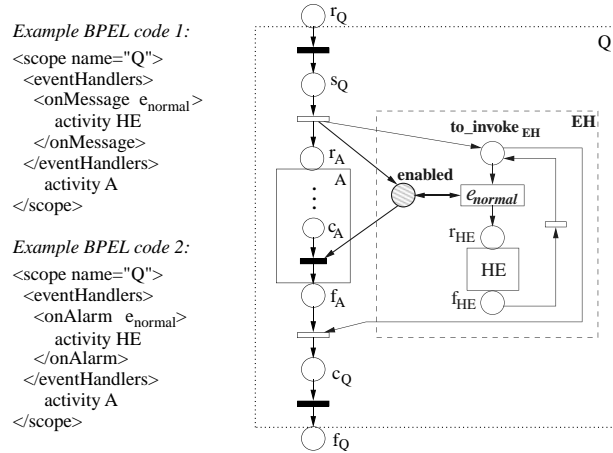
Fig. 8. Mapping event handlers.
