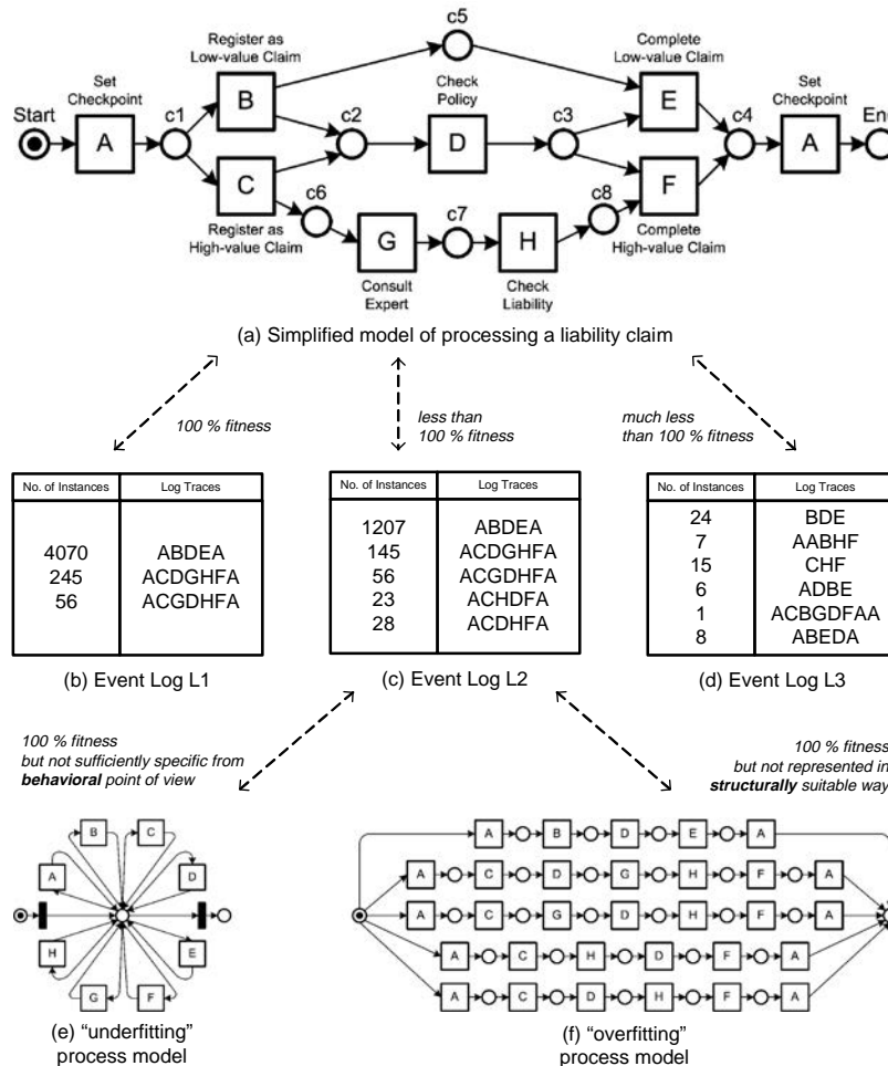
Fig. 3. Two dimensions of conformance: fitness and appropriateness.
