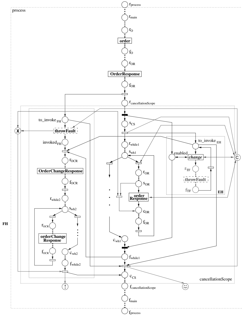
Fig. 9. Mapping of the Supplier process shown in Figure 5.
