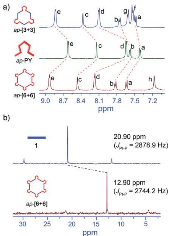
Fig. 3 Characterization of hexagon ap-[3 + 3] and ap-[6 + 6]. (a) Partial ^1\text{H} NMR spectra (400 MHz, 293 K) of ap-[3 + 3], ap-PY and ap-[6 + 6] in a mixture of \text{CD}_2\text{Cl}_2 and \text{acetone-}d_6 . (b) ^{31}\text{P} NMR spectra (161.9 MHz, \text{CD}_2\text{Cl}_2 , 293 K) of 180° di-Pt(II) acceptor 1 and ap-[3 + 3].
