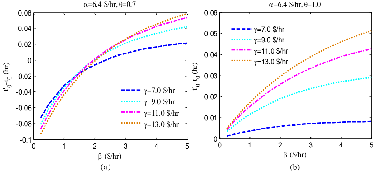
Figure 8 Difference between the earliest departure time with a single step coarse toll and that with no toll
