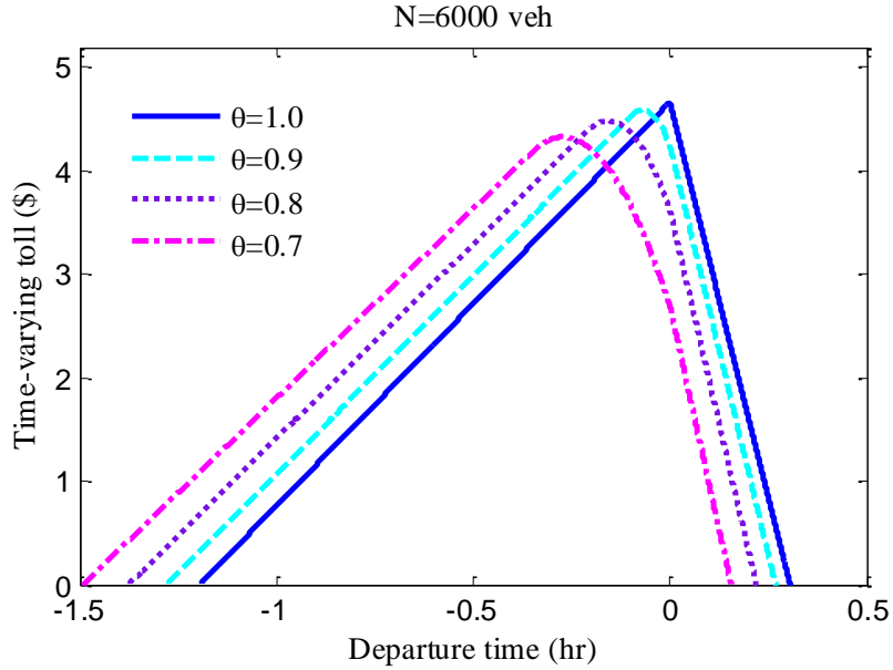
Figure 6 Time-varying toll for different \theta values
