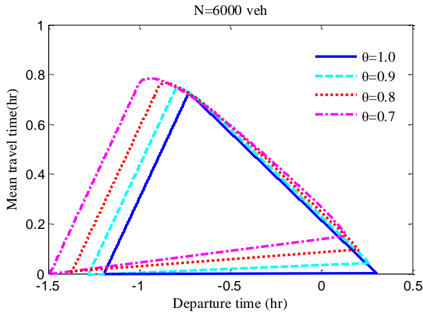
Figure 5 Travel time distributions with departure time under no-toll (the upper concave profiles) and time-varying toll (the lower linear distributions)
