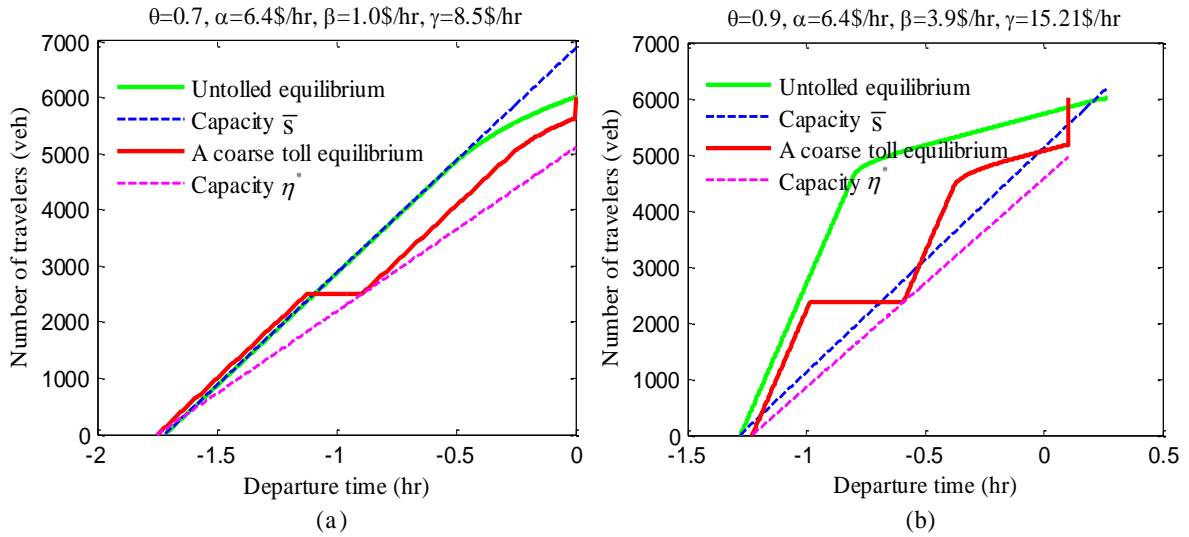
Figure 9 Cumulative departures with different parameters of single-step coarse toll in equilibrium
