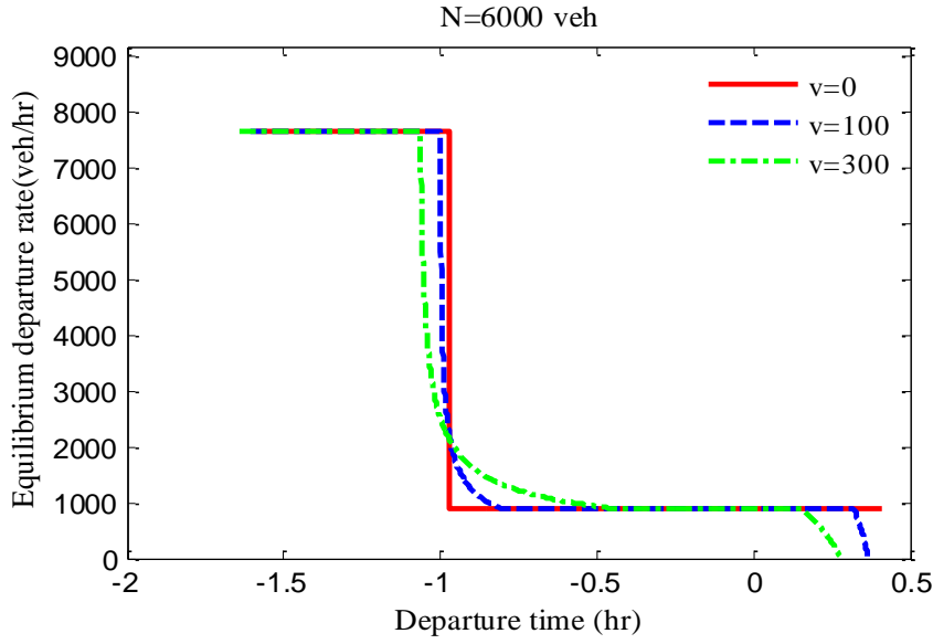
Figure 4 Equilibrium departure rate for different v values
