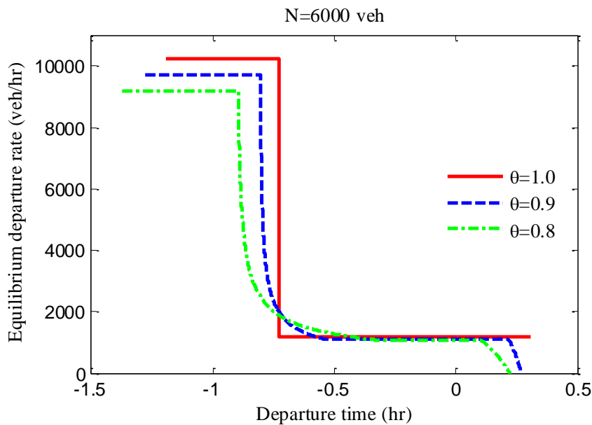
Figure 3 Influence of parameter \theta on departure rate
