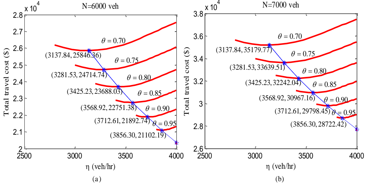
Figure 7 Total travel cost for different \theta and N values
