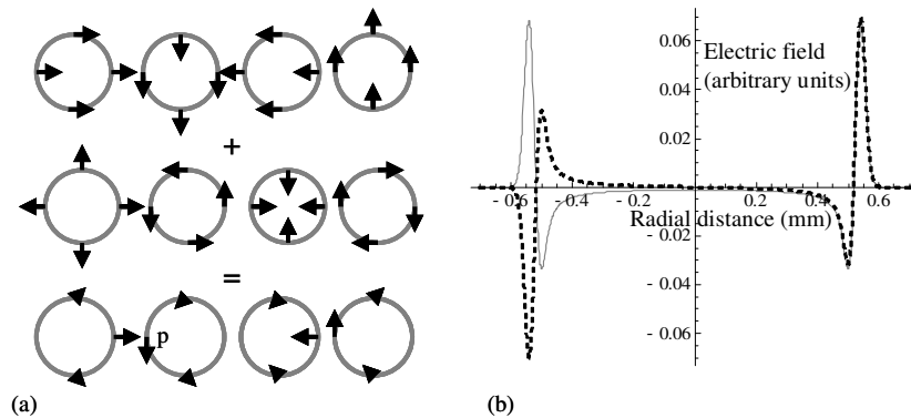
Fig. 5. The different phase properties of the fields described by B_0 & B_1 . 5(a) shows, over one optical cycle, the how field vectors of the B_0 component combine with the field vectors of the B_1 field to give the half turn of polarization associated with conical refraction; 5(b) shows a snapshot of the B_0 and B_1 electric field profiles in the focal image plane ( B_1 dashed)
