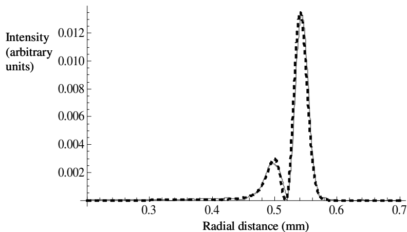
Fig. 7. A comparison of experiment with theory (dashed line) in the focal image plane; Radial distance is measured from the centre of the cylinder associated with conical refraction (Fig. 1)
