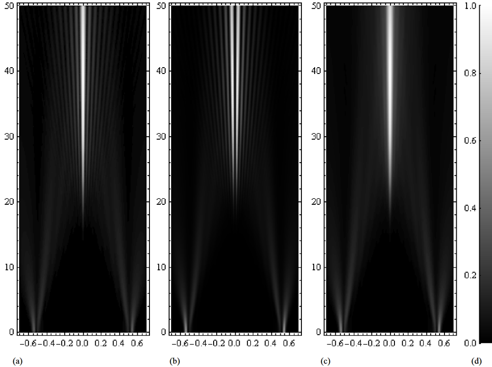
Fig. 2. The intensity due to B_0 (a), B_1 (b) and the conically diffracted Gaussian field, B_0 + B_1 (c) as the beam propagates away from the focal image. The vertical axis measures distance from the focal image plane in mm and the horizontal axis measures radial distance in mm. (d) shows the normalized greyscale.
