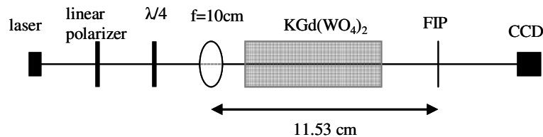
Fig. 6. This optical arrangement used to analyze conical diffraction requires no imaging lens
