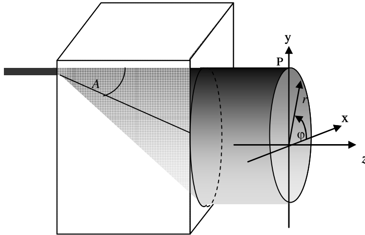
Fig. 1. The system of cylindrical co-ordinates used to describe the cylinder of light that propagates in space after having been refracted into a cone of semi-angle A within the crystal.
