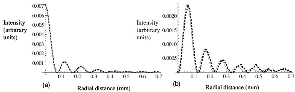
Fig. 9. (a) Exact far field B_0 vs experimental data (dashed) at 10.75 cm from FIP; (b) same data for B_1
