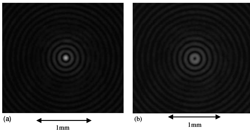
Fig. 8. CCD pictures of diverging Bessel beams; B_0 in (a); B_1 in (b)
