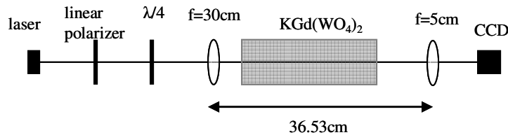
Fig. 10. Optical setup for non-diverging Bessel beams
