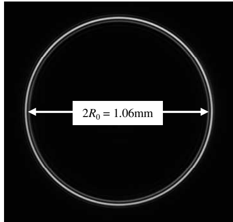
Fig. 4. Experimental image of the focal image plane, the excellent quality of the crystal is obvious from the image above
