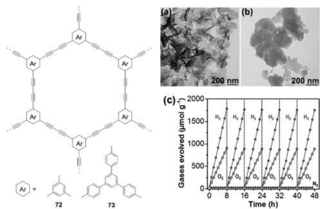
Fig. 17 Chemical structures of polymers 72 and 73 ; TEM pictures of (a) 72 and (b) 73 as well as (c) time course of H 2 and O 2 production of polymer 73 . Reprinted with permission from ref. 40. Copyright 2017 Wiley-VCH.
